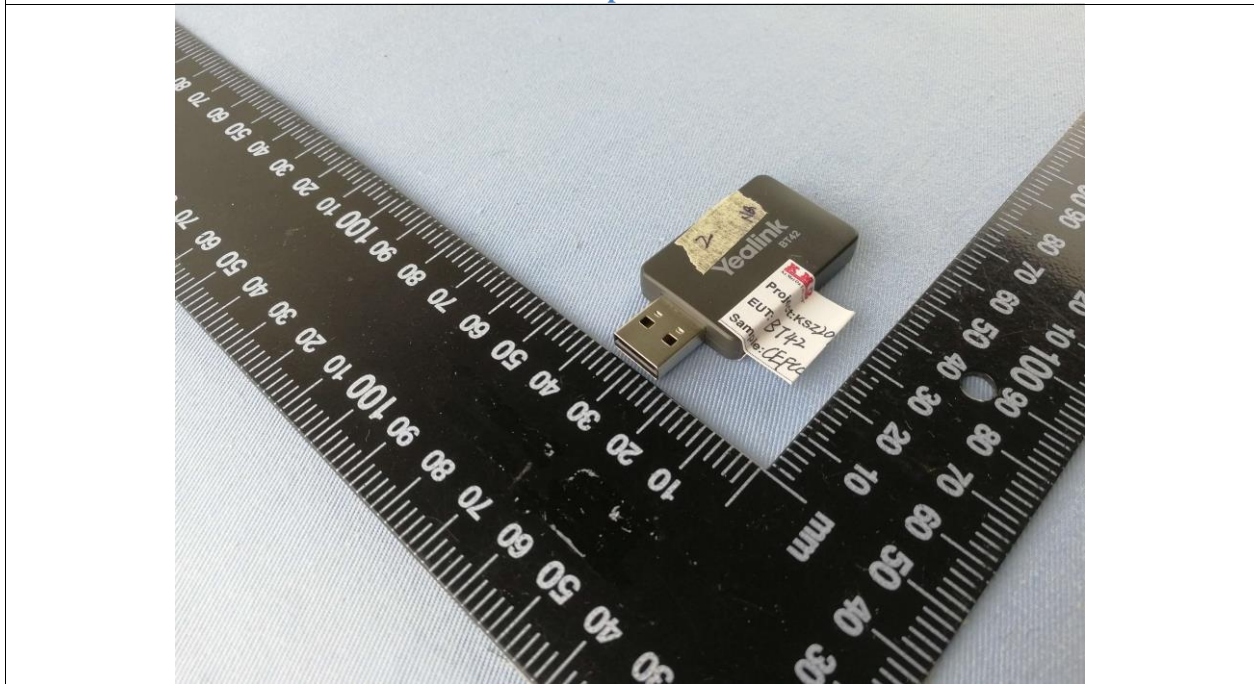
EUT top side view
