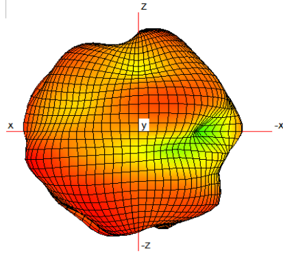
2.44GHz X-Z plane View
