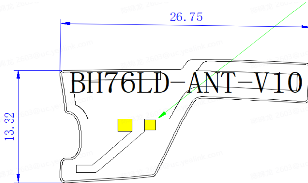
Antenna Dimensions
