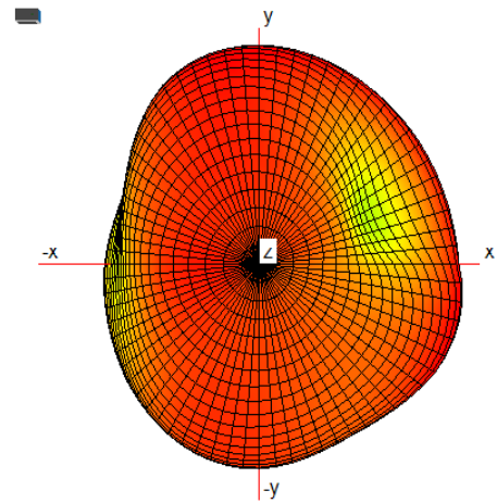
3D Antenna pattern
