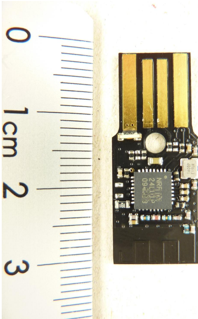
125162_18.JPG: PCB, top view
