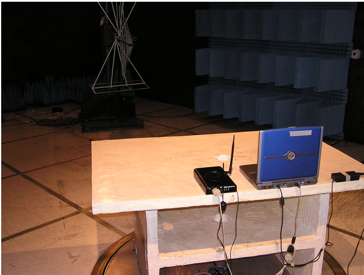
RADIATED EMISSIONS
