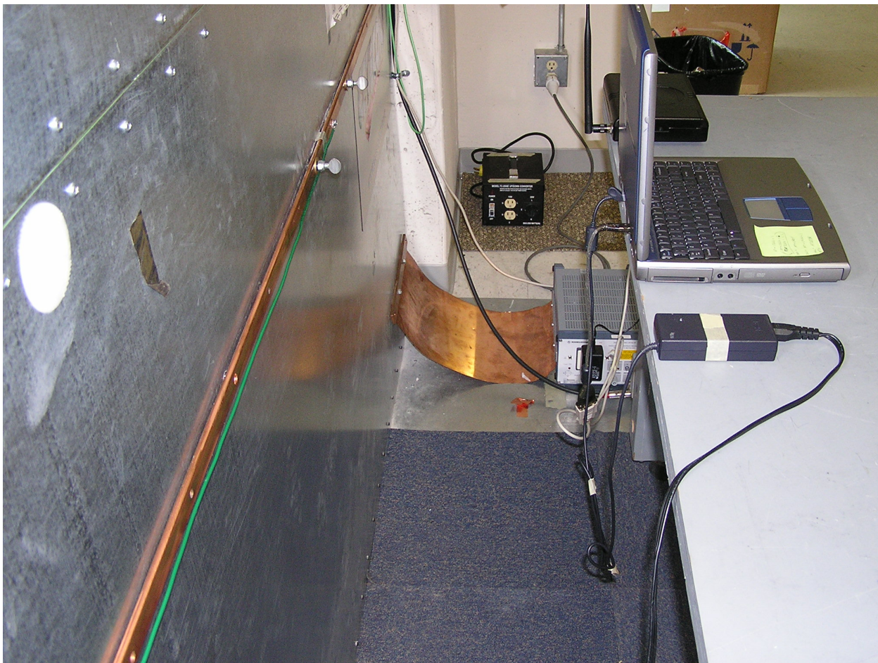
AC POWERLINE CONDUCTED EMISSIONS
