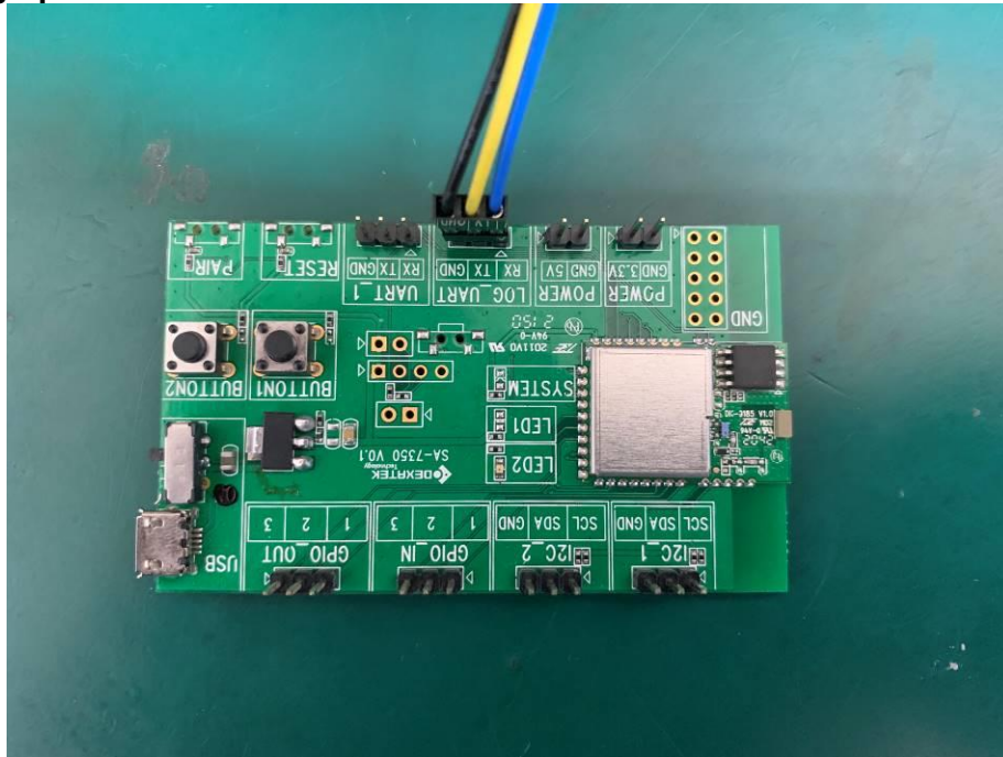
Photograph 9: Fixture
