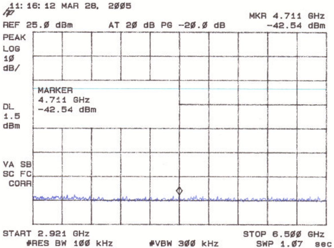
Figure 4g Antenna Conducted Spurious Emissions 15.247(c) (Mid Channel)
