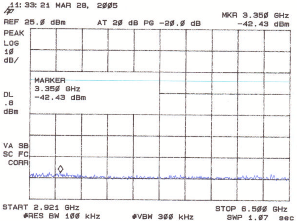
Figure 4k Antenna Conducted Spurious Emissions 15.247(c) (High Channel)
