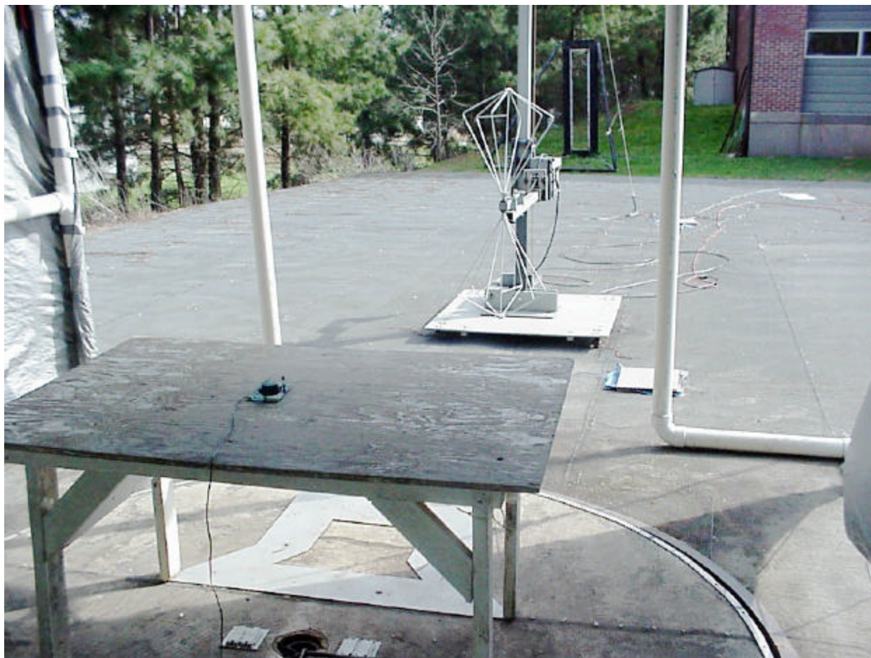
Photograph represents worst case configuration
