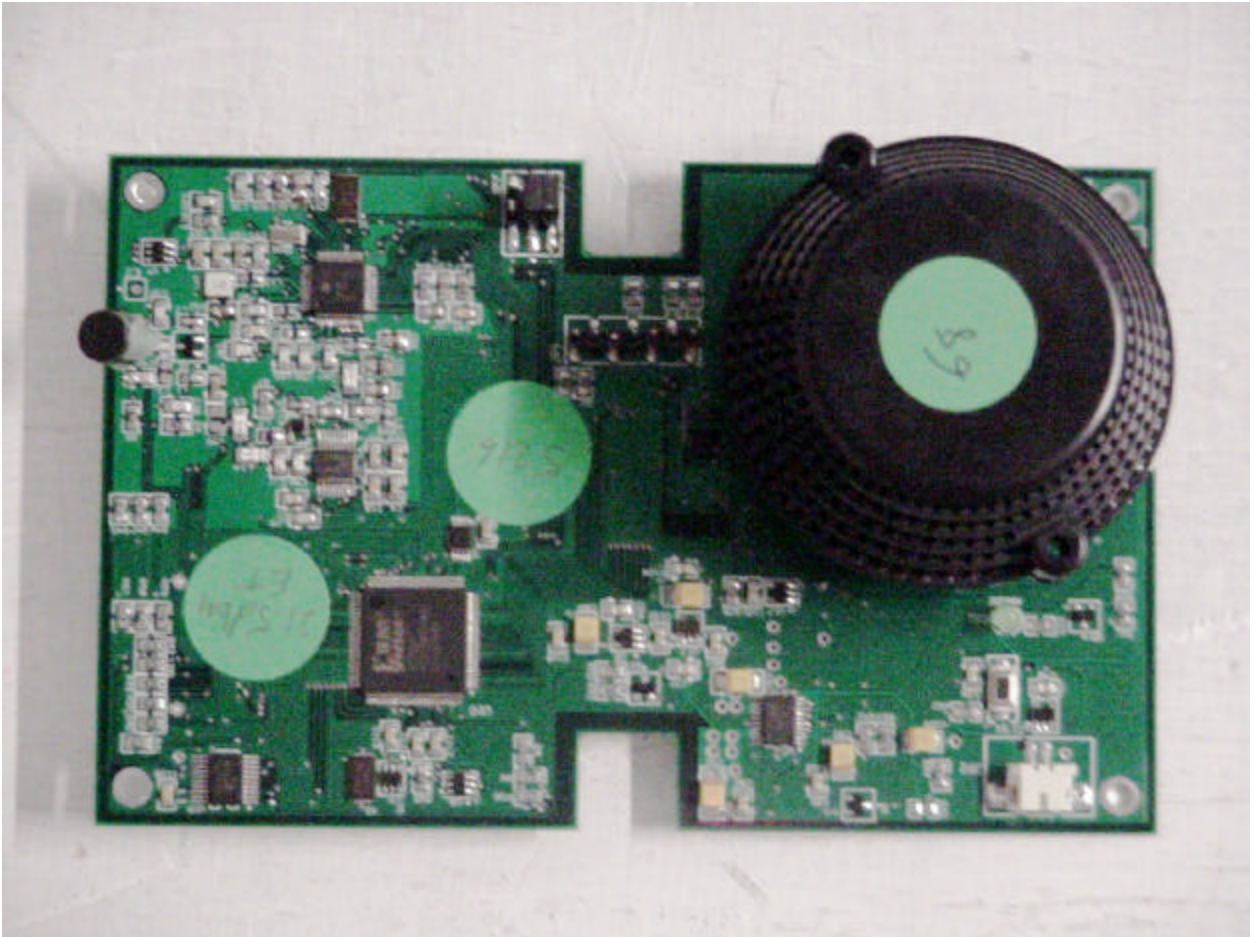
Photo 1. EUT, Top with Daughter Board
