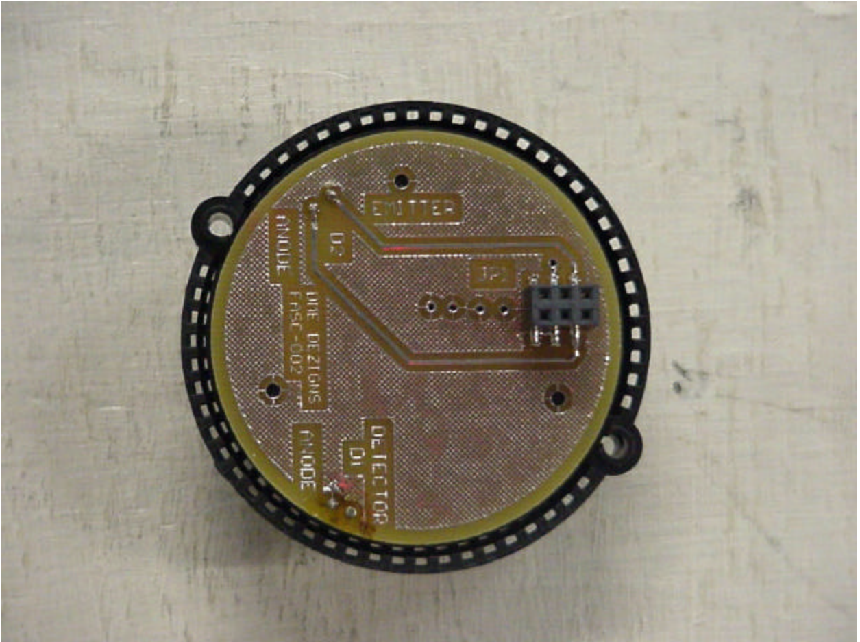
Photo 4. Daughter Board, Bottom
