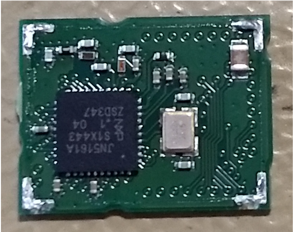
Figure 1: Top view of module without shield
