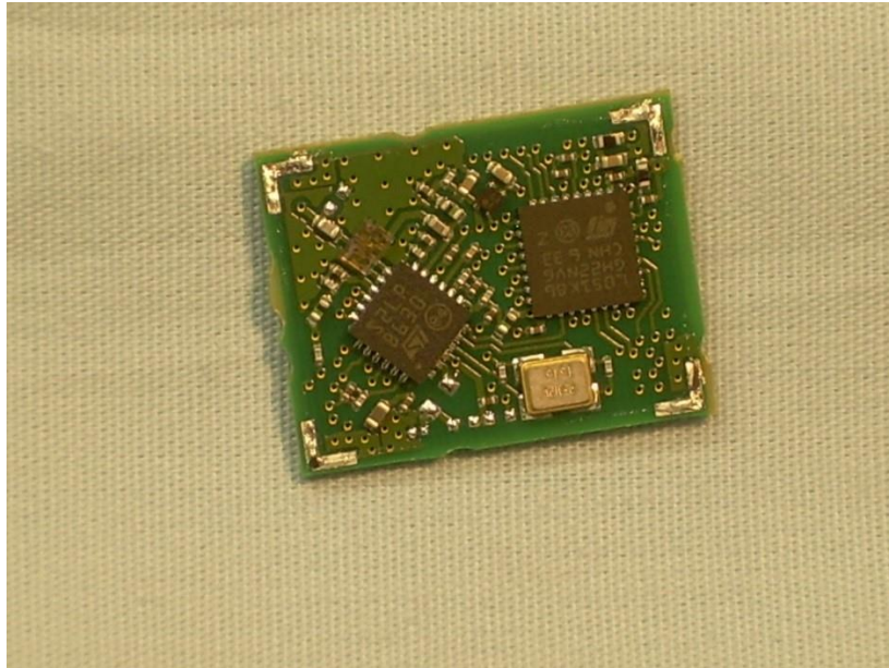
Photograph 3 – Top View of the EUT – RF Shield Removed Showing Components Underneath
