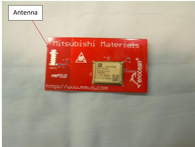
Photograph 5 – Front View of the EUT – Chip Antenna
