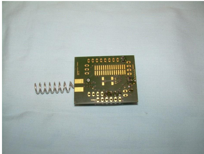
Photograph 4 – Back View of the EUT – Helical Antenna
