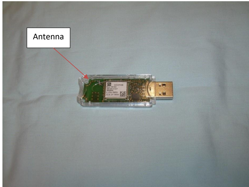
Photograph 9 – Front View of the EUT – Trace Antenna
