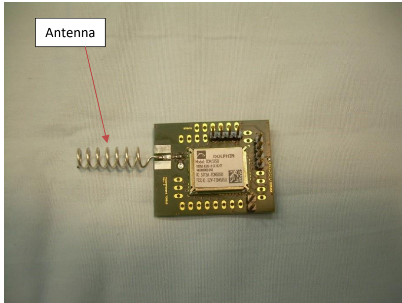
Photograph 3 – Front View of the EUT – Helical Antenna
