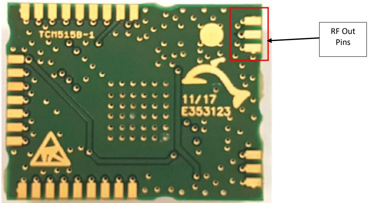
Photograph 2 – Back View of EUT
