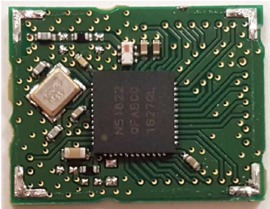
Photograph 1 – Front View of EUT, without RF Shield
