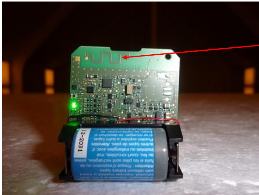
Photograph 2 – Back View of Carrier Board
