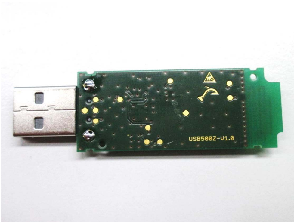
Photo A3-4: Demo-Board USB500Z-V1.0 with soldered EUT – Bottom view
