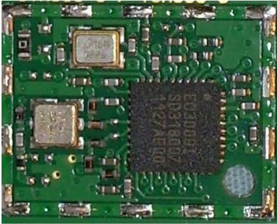
Circuitry Under RF Shield
