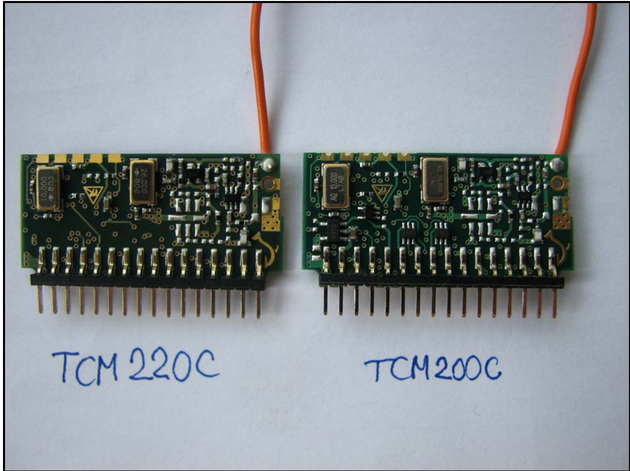
Photograph 6: Bottom View
