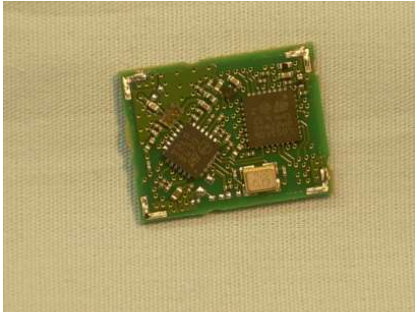
Photograph 17: Circuitry Under RF Module Shield
