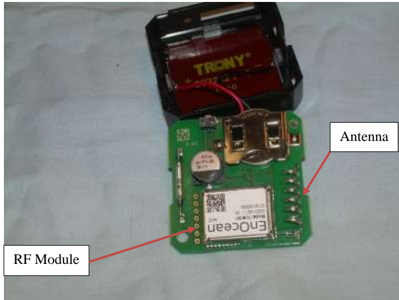
Photograph 15: Side A of PCB
