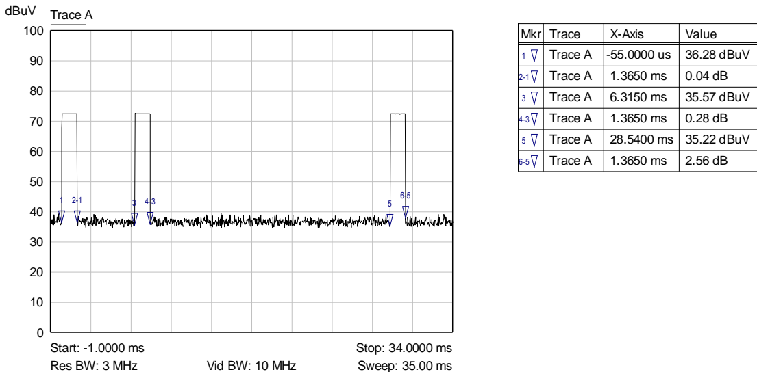
Graph 4: Plot over 35 ms time period
