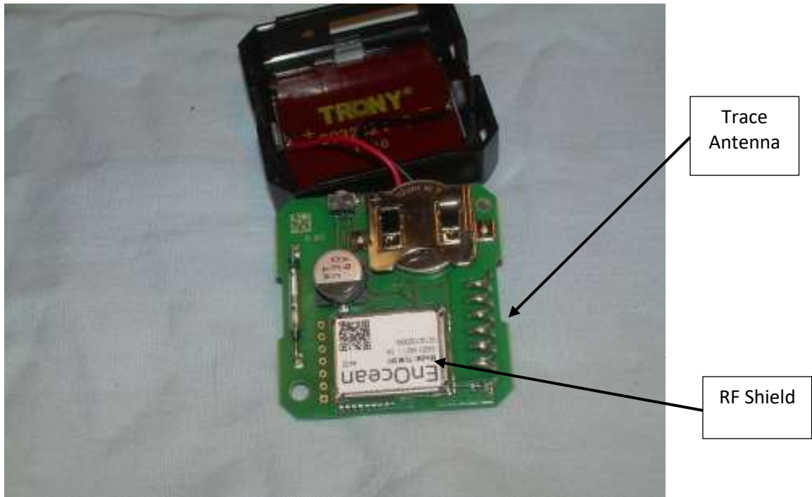
Photograph 1 – Front View of the Device
