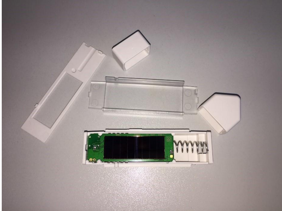
Photograph 1 – View of the EUT Housing Parts
