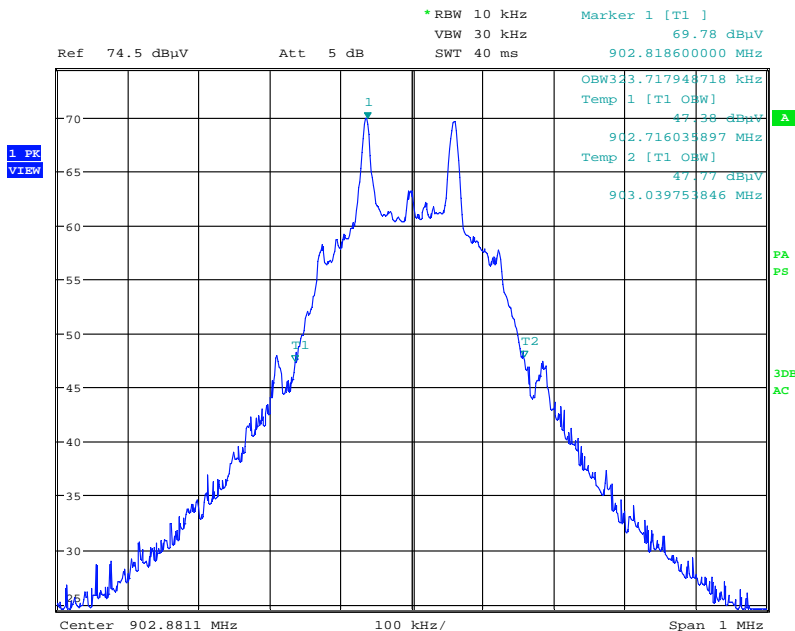
Plot 8.5-1: EUT STM 332U, sample 1, bandwidth plot – 20 dB bandwidth
