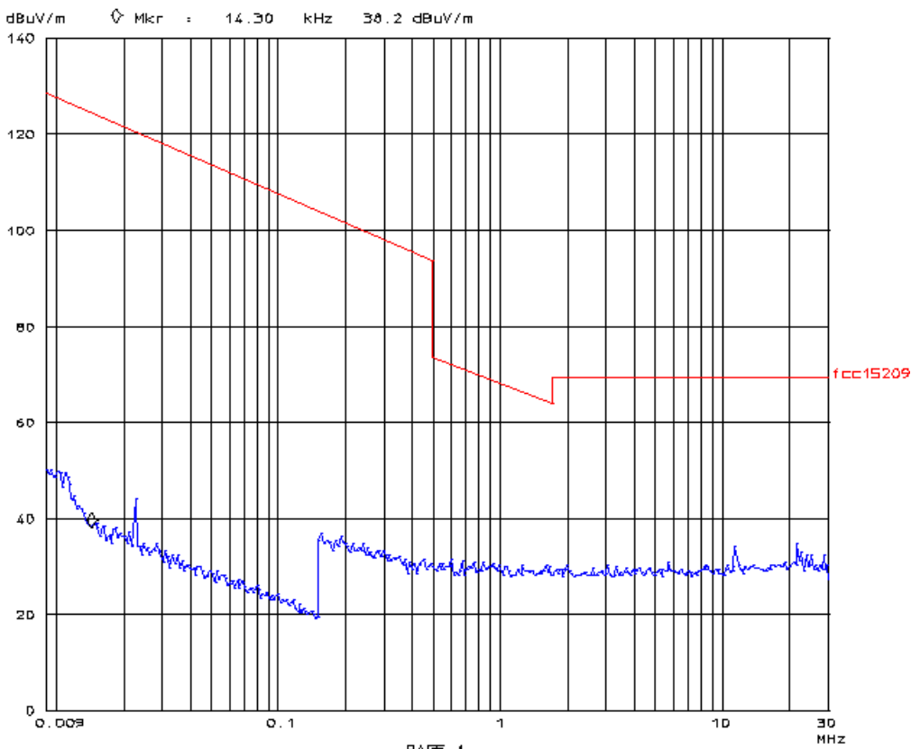
Plot 6.7.2.1: EUT STM 332U, sample 1, Magnetic Field emissions at 3m distance
