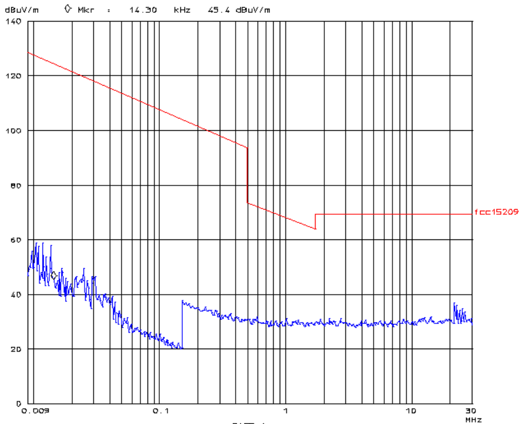
Plot 6.7.2.2: EUT STM 333U, sample 1, Magnetic Field emissions at 3m distance
