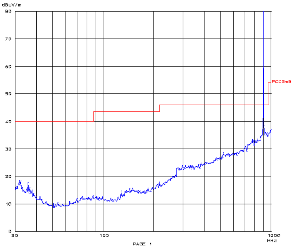
Plot 6.7.3-1: EUT STM 332U, sample 1, pre-scan plot d = 3m (30 MHz to 1 GHz)
