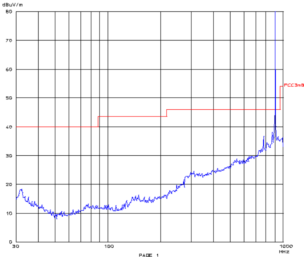
Plot 6.7.3-2: EUT STM 333U, sample 1, pre-scan plot d = 3m (30 MHz to 1 GHz)
