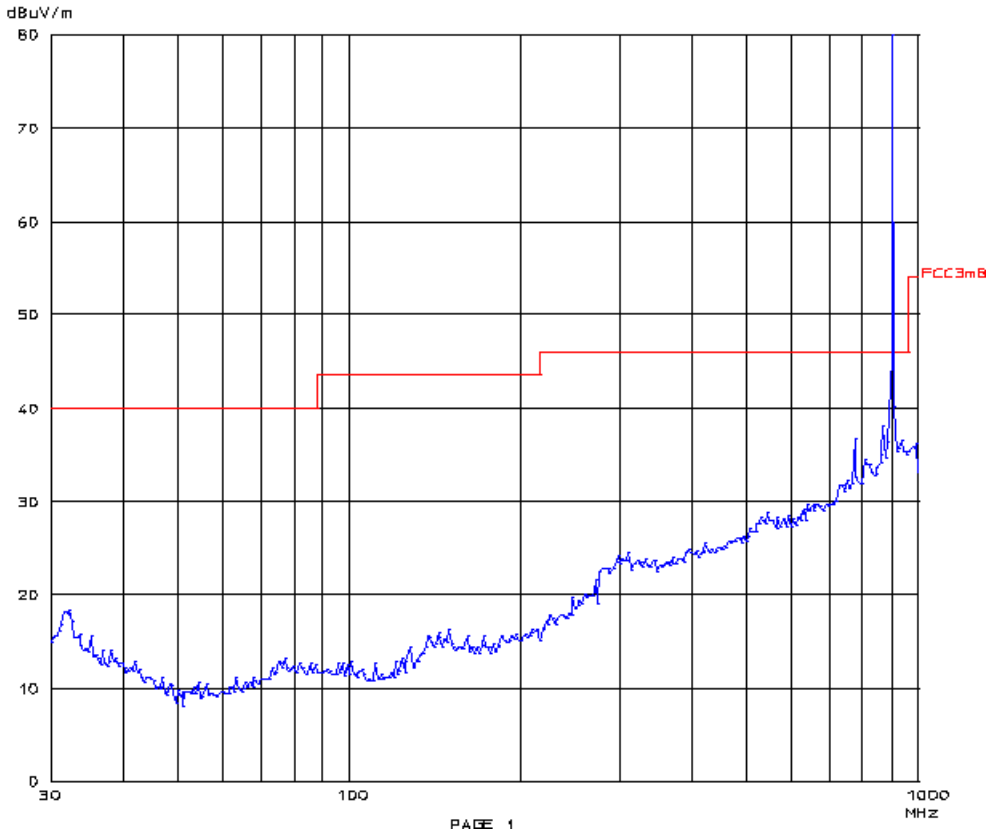
Plot 6.7.3-1: EUT STM 333U, sample 1, pre-scan plot d = 3m (30 MHz to 1 GHz)
