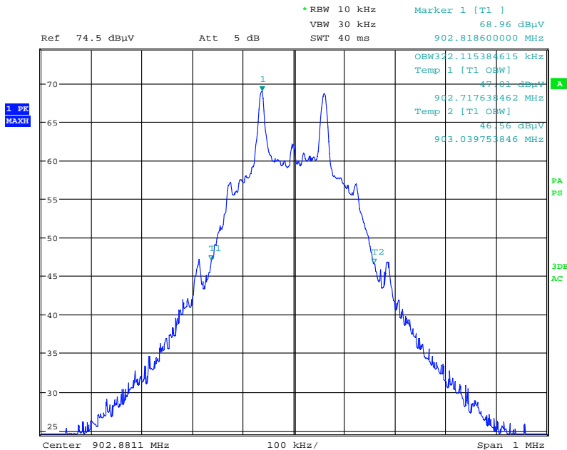
Plot 8.5-3: EUT STM 333U, sample 1, bandwidth plot – 20 dB bandwidth
