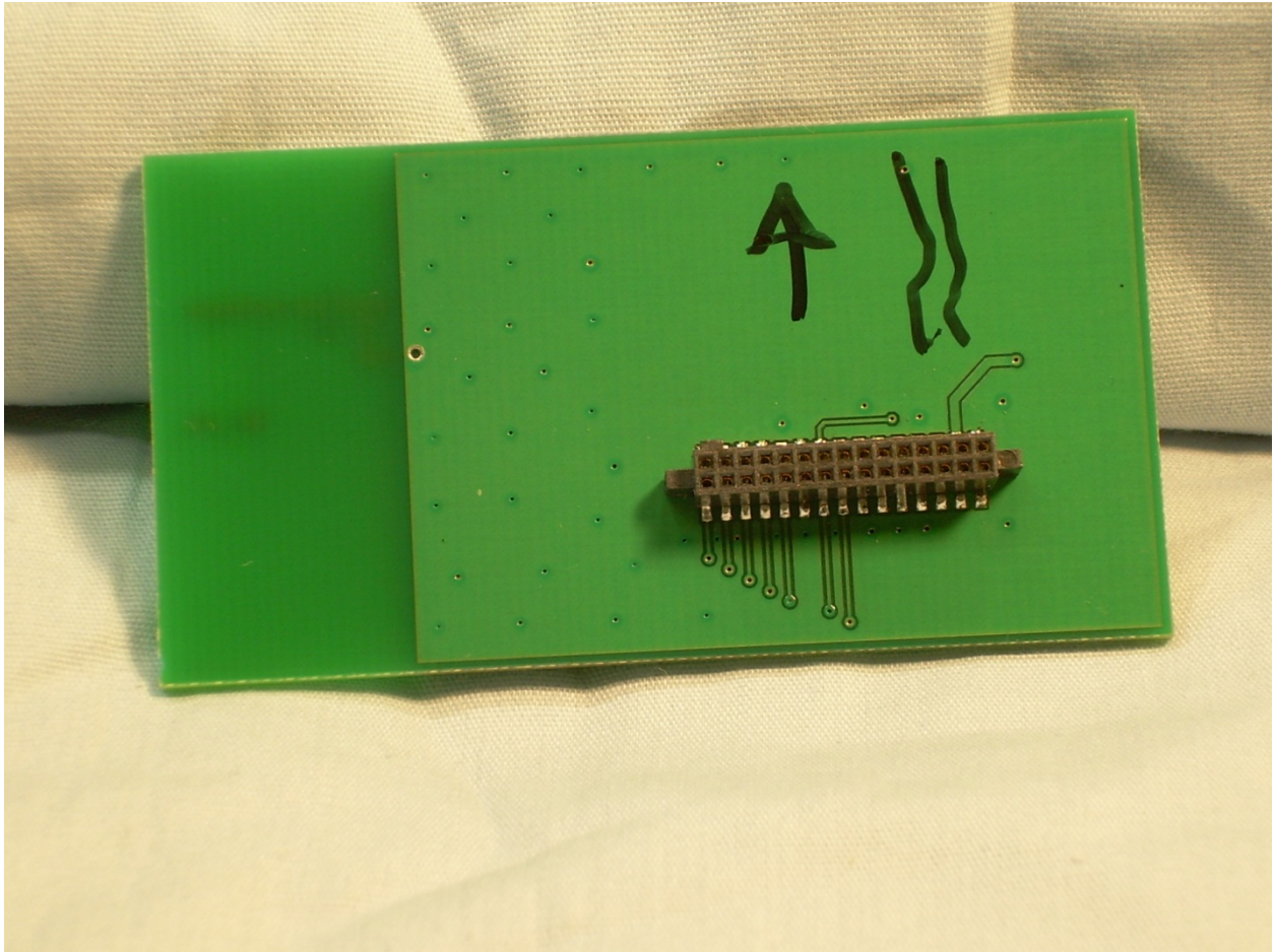
Back View of the PCB with Module Interface Connector
