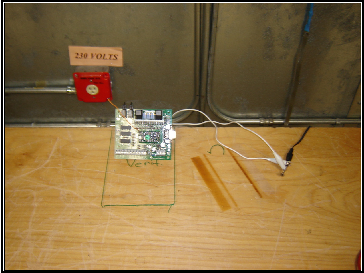
Photograph 3: AC Line Emissions
