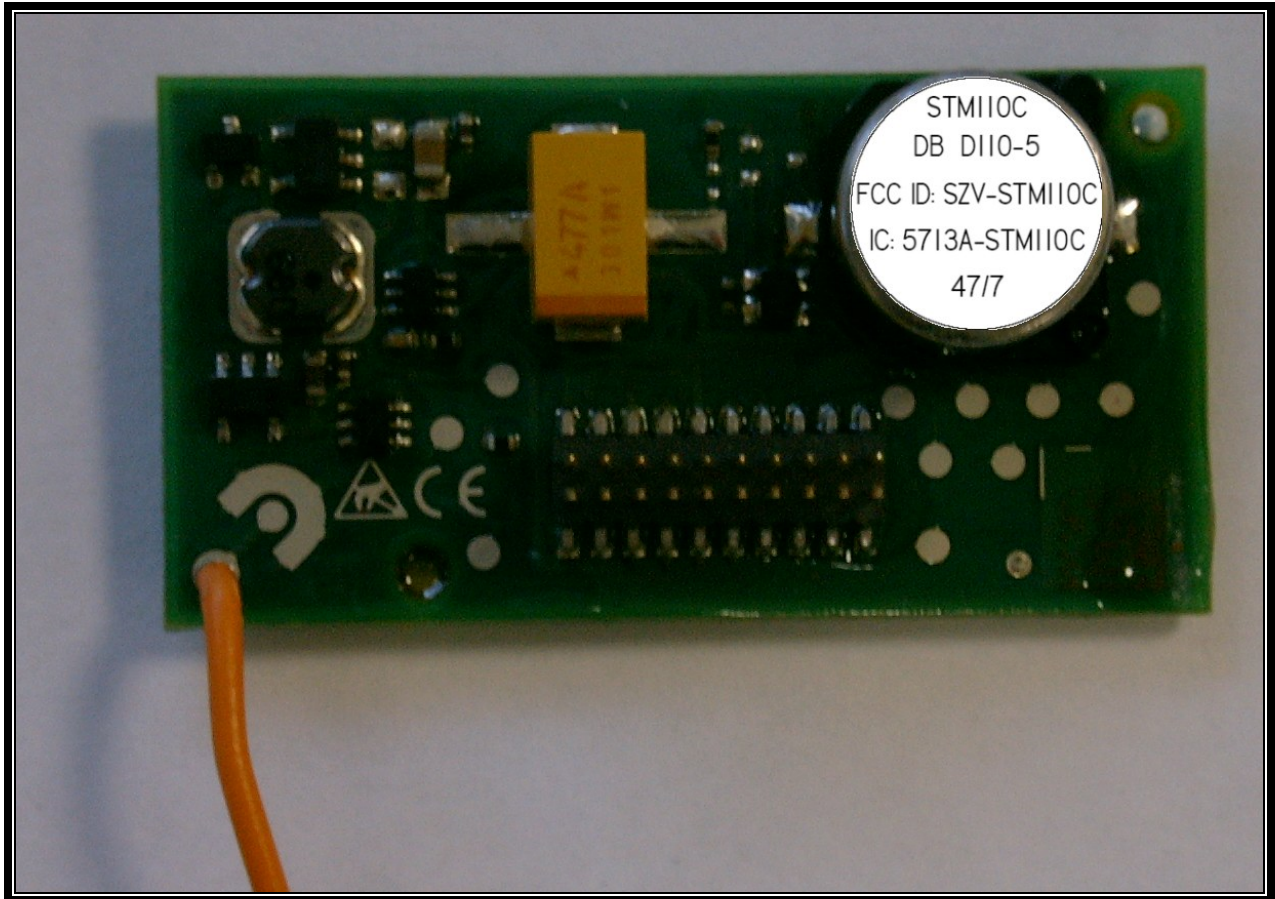
Photograph 5: Radio PCB - Back View
