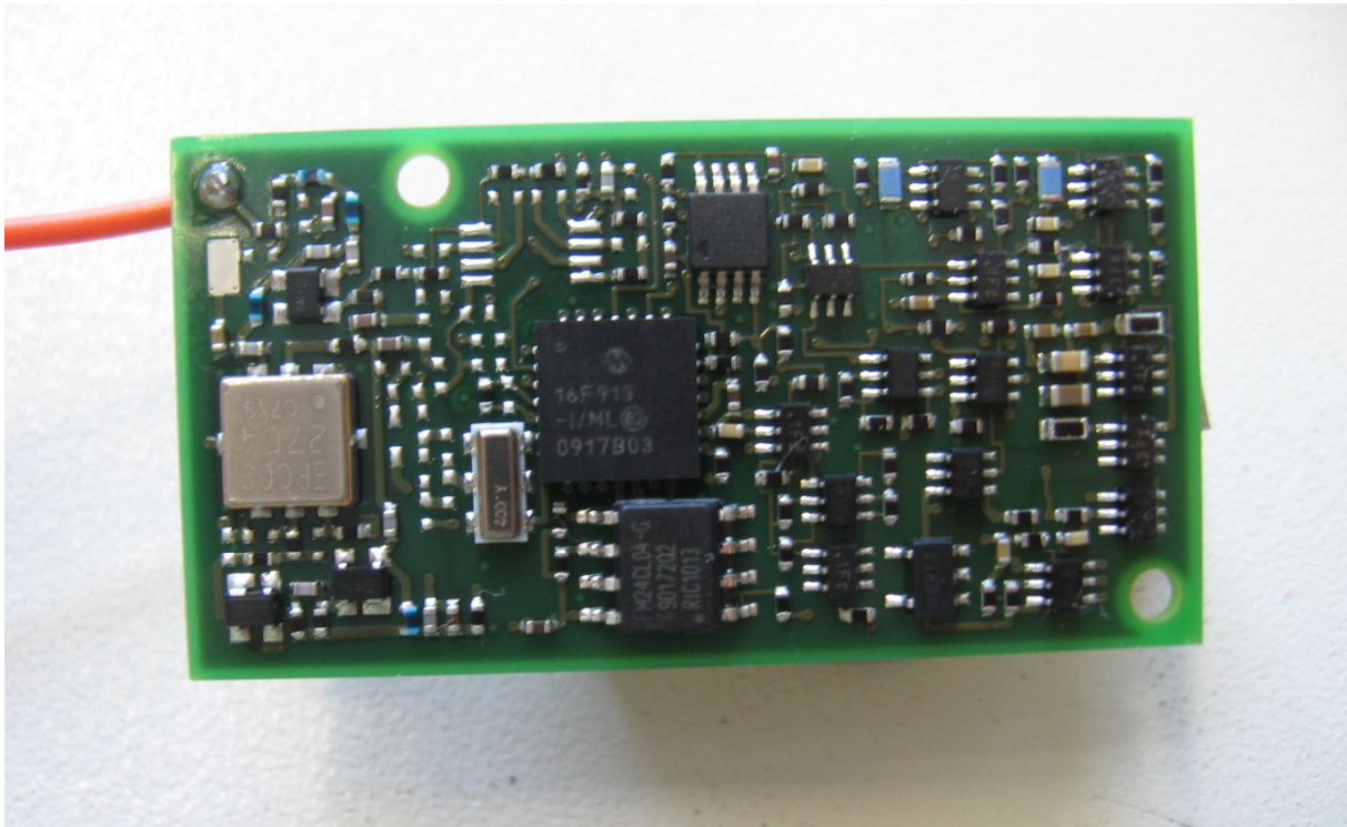
Radio PCB – Front View
