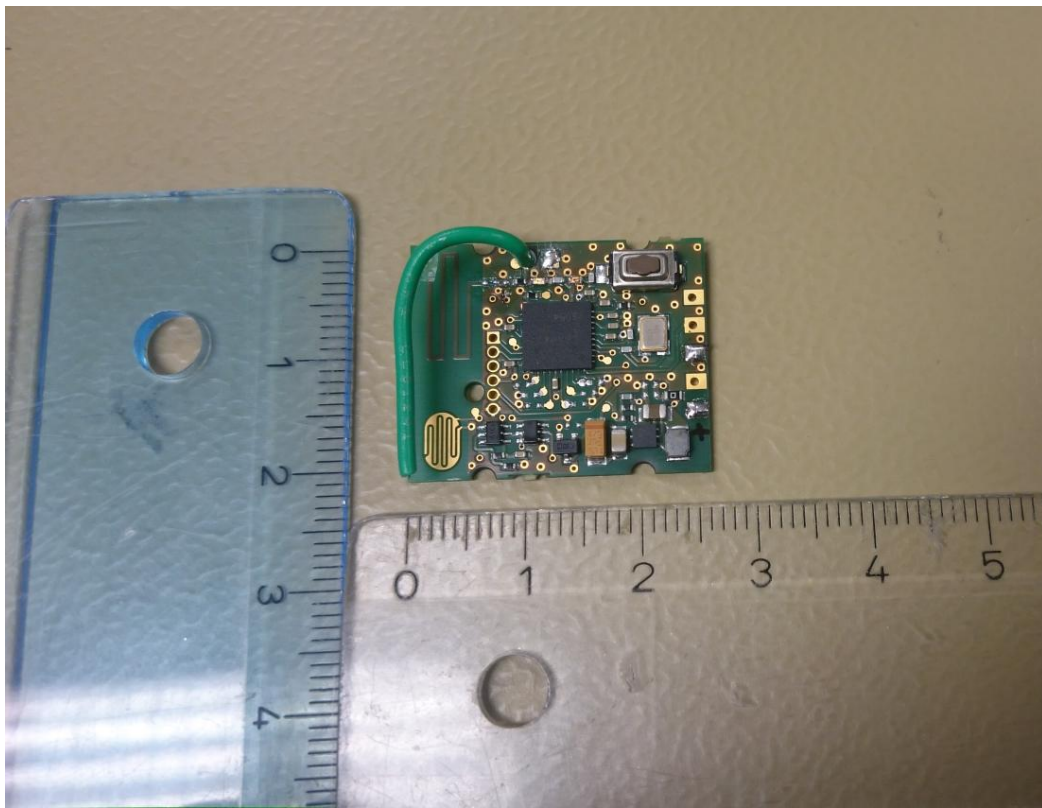
Top side with external antenna
