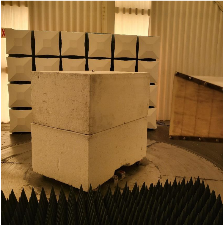
Photograph 3: Front View Radiated Emissions Worst Case – Above 1000 MHz Configuration
