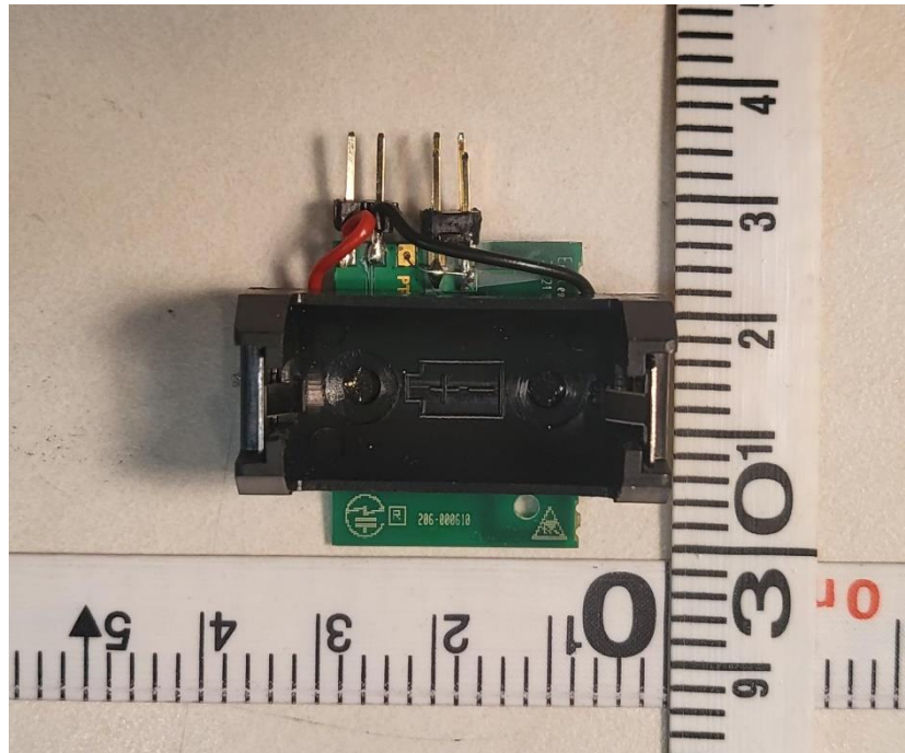
Photograph 3 – Back View of the EUT
