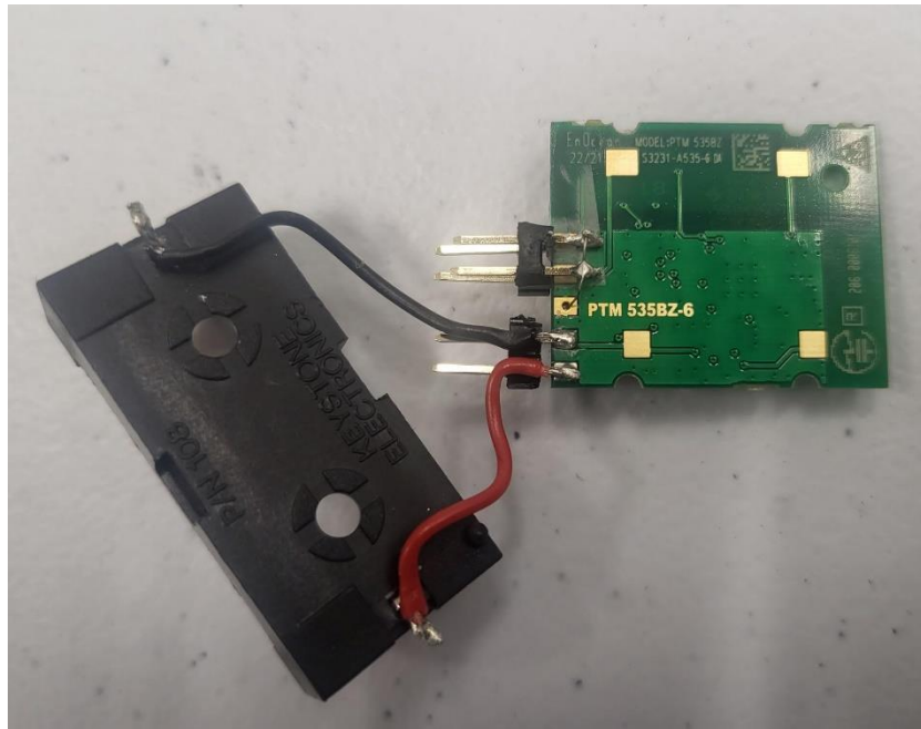
Photograph 7 – View of PCB with Battery Holder Removed
