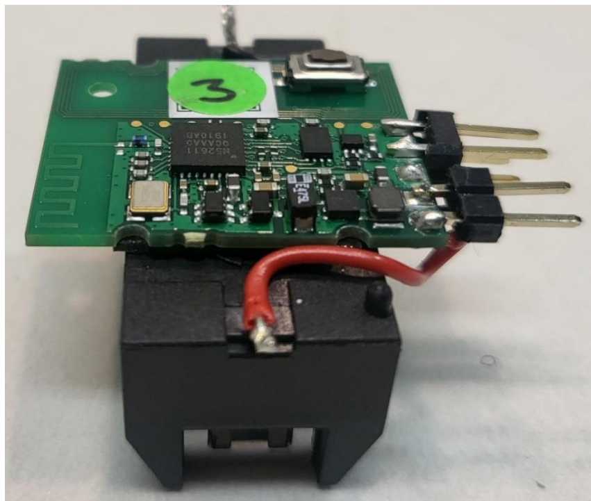
Photograph 2 – Edge1 View
