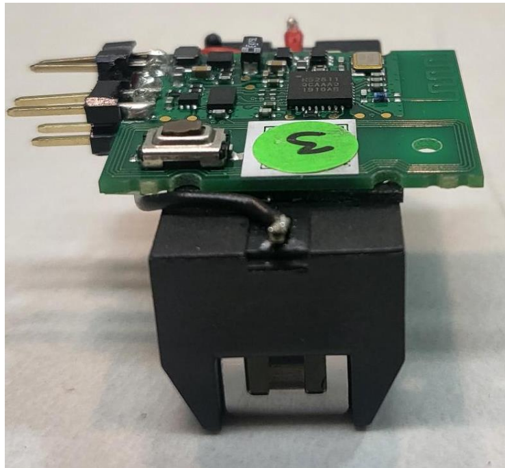
Photograph 5– Edge3 View
