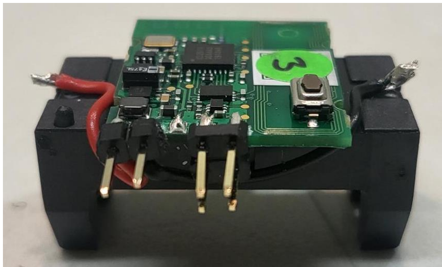
Photograph 6 – Edge4 View
