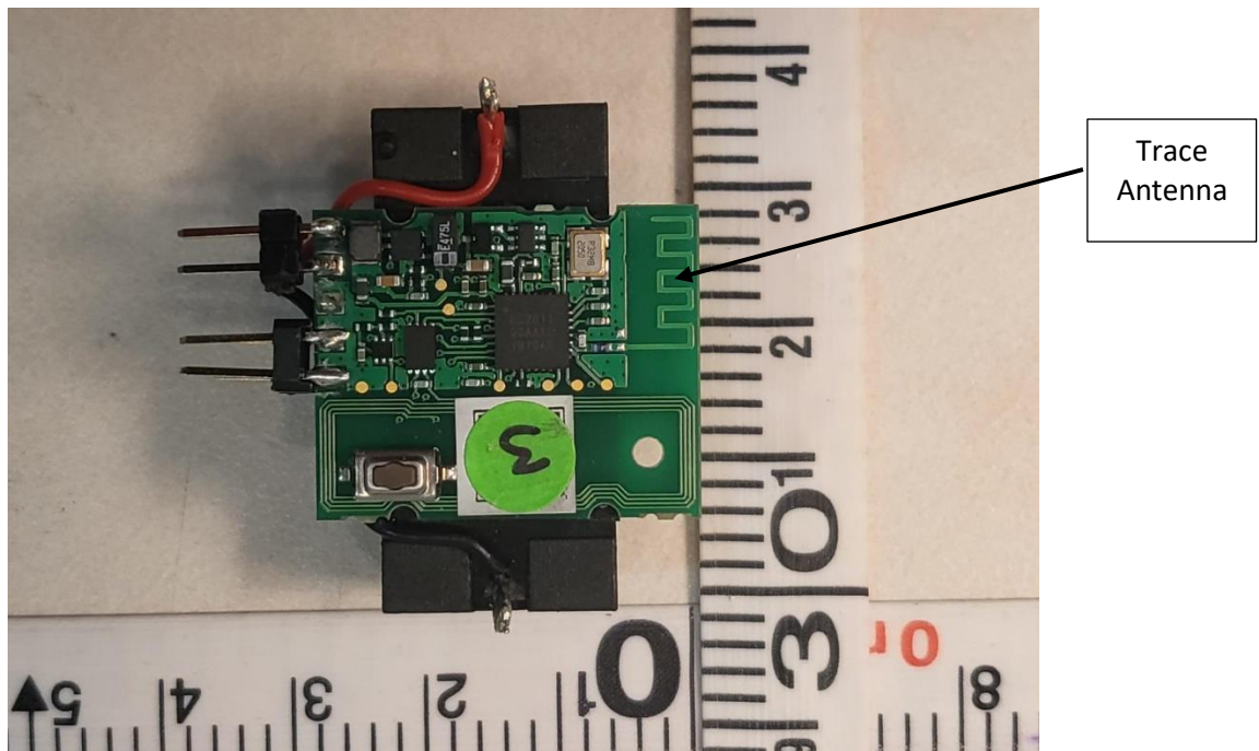
Photograph 1 – Front View of the EUT
