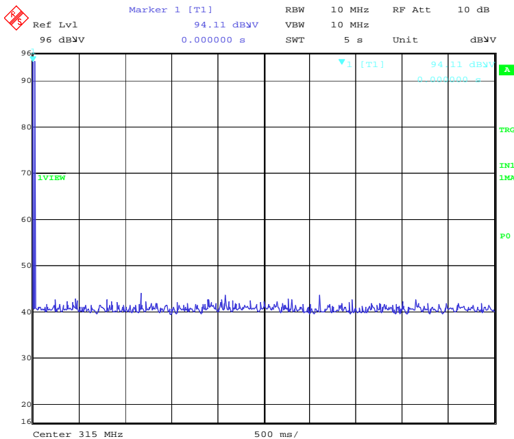
Plot 7.2.2: EUT sample 3, duration of transmission
