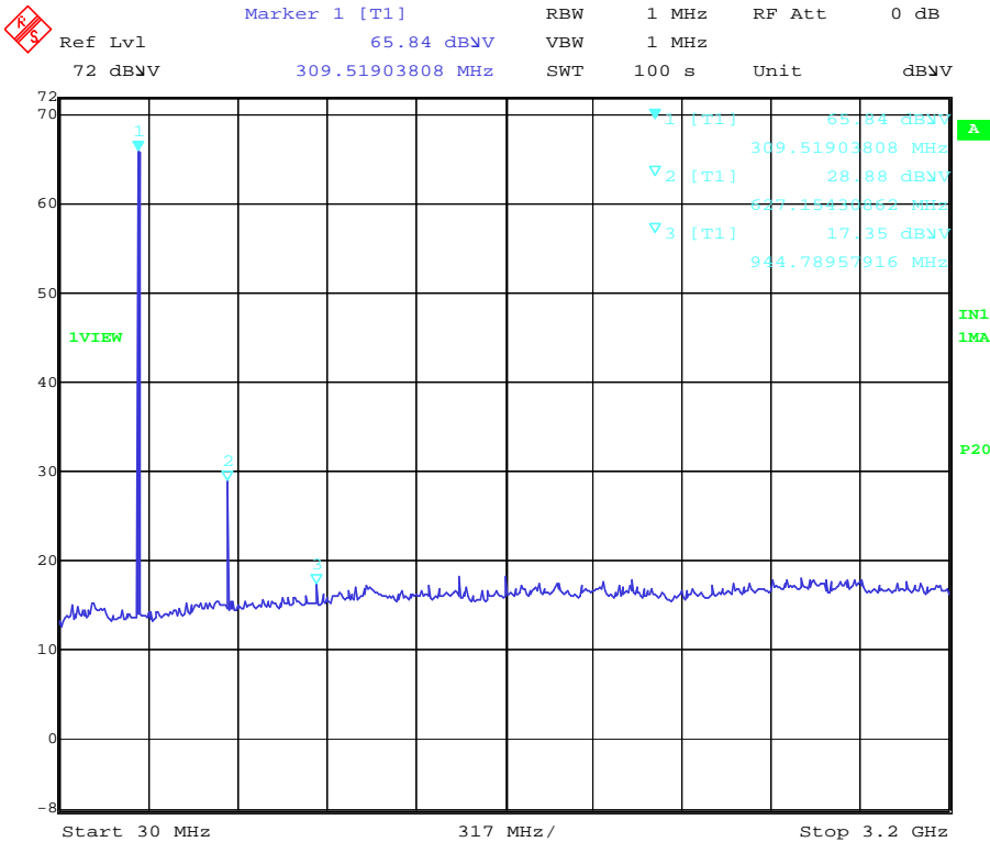
Plot 6.7.3-1: EUT sample 4, pre-scan plot d = 3m (30 MHz to 3.2 GHz)
