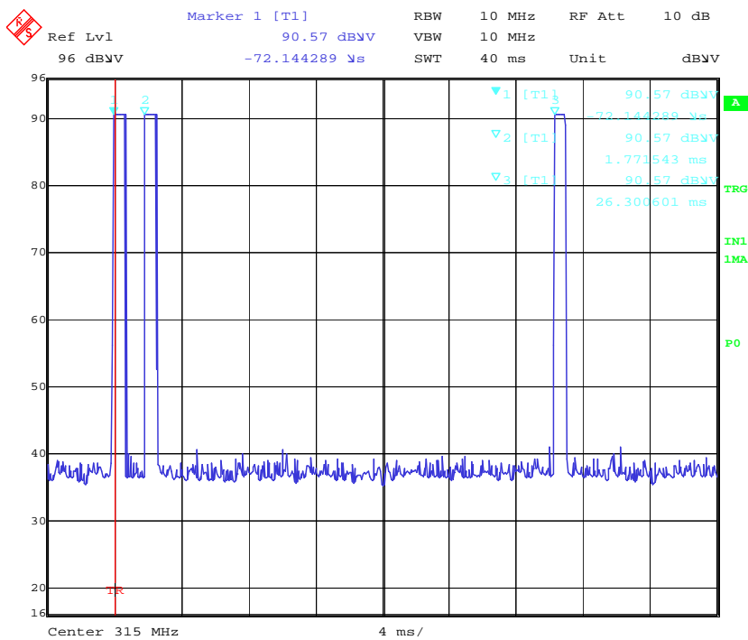
Plot 6.7.1-1: EUT sample 3, Complete transmission pattern after starting at line TR (= video trigger)
