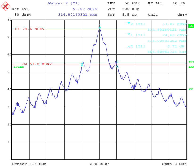
Plot 8.5-1: EUT sample 4, bandwidth plot – 20 dB bandwidth
