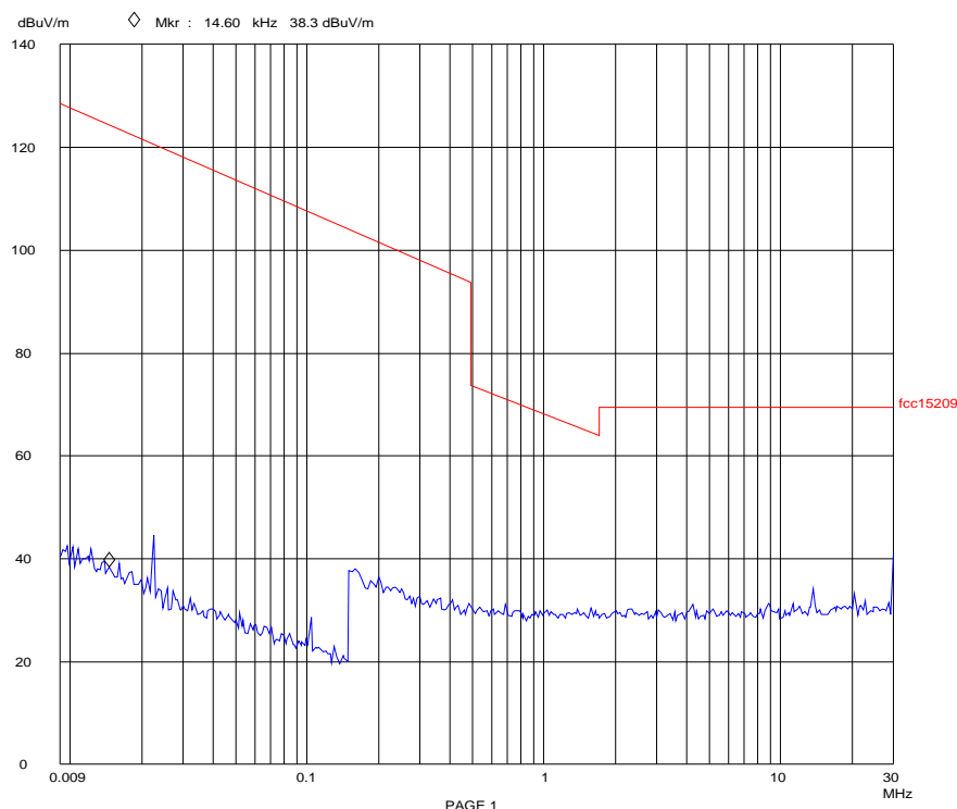
Plot 6.7.2: EUT sample 4, Magnetic Field emissions at 3m distance
