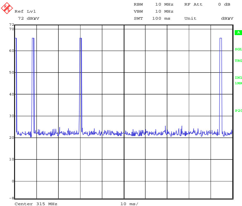
Plot 6.7.1-2: EUT sample 3, duration of one block, duty cycle - ton = 3 * 773 μs; T = 100 ms → duty cycle = 0.0232 (= -32.7 dB)
