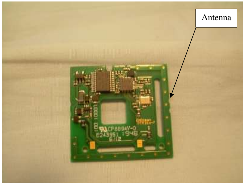
Photograph 14 – View of the Component Side of the PCB
