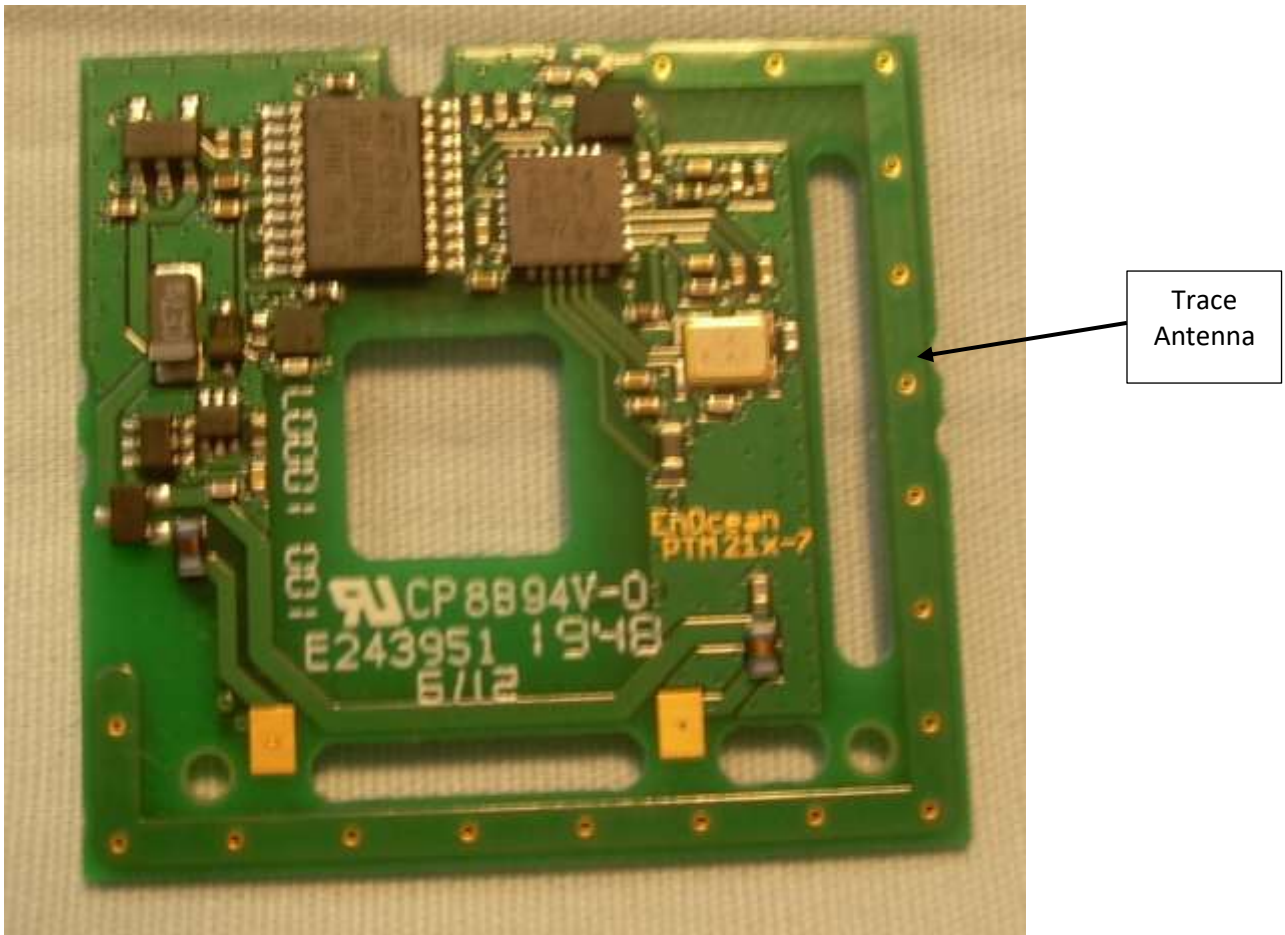
Photograph 1 – Front View of the Device
