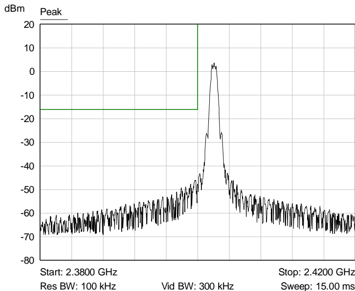
Graph 7: Lower Band Edge Plot
