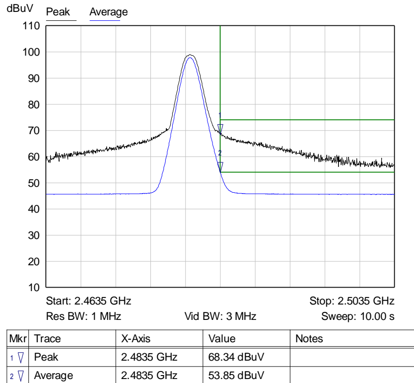
Graph 23: Radiated Upper Band Edge Plot
