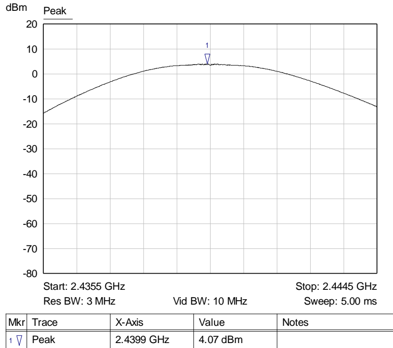
Graph 18: Middle Channel Output Power
