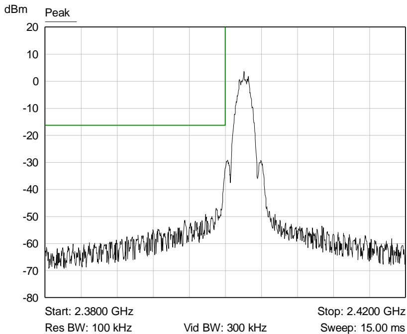
Graph 20: Lower Band Edge Plot
