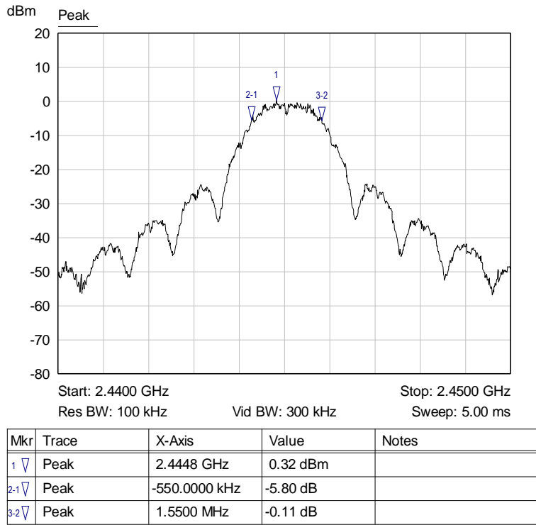
Graph 28: Middle Channel Bandwidth
