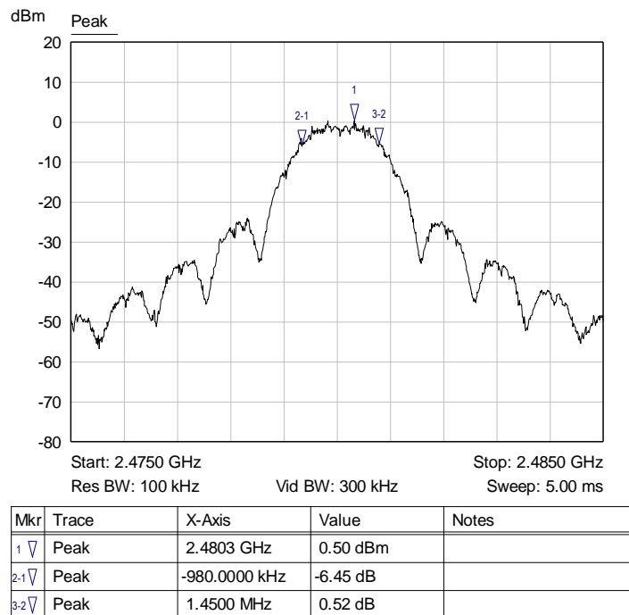
Graph 29: Highest Channel Bandwidth
