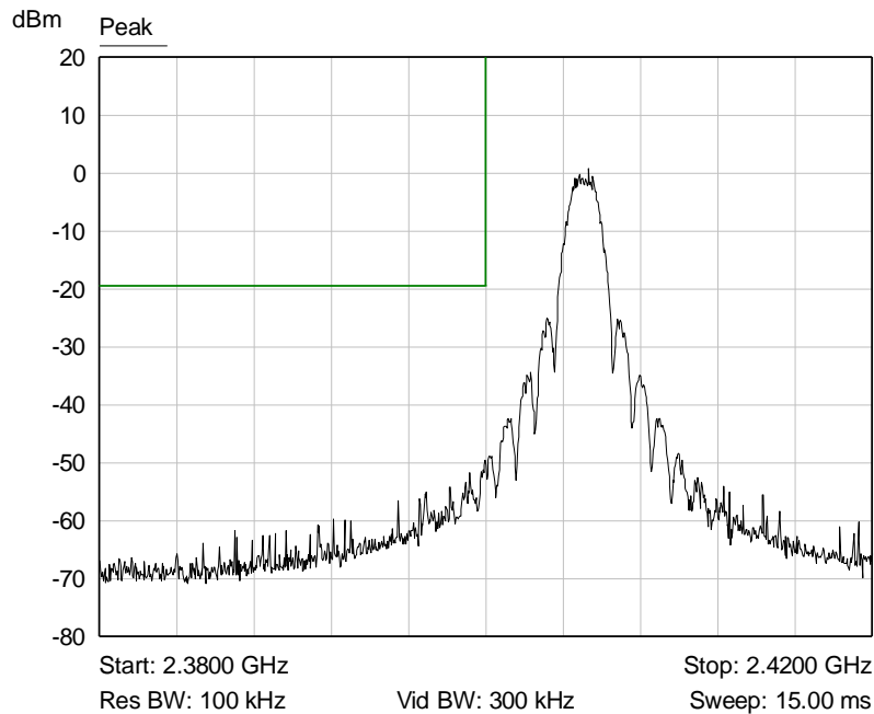
Graph 33: Lower Band Edge Plot
