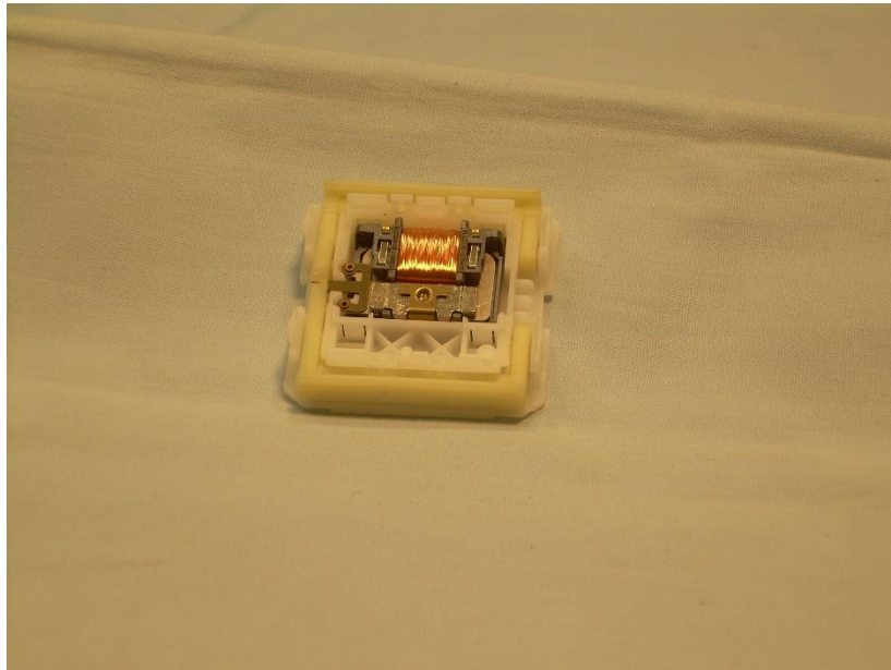
Photograph 16: View of the Energy Generator
