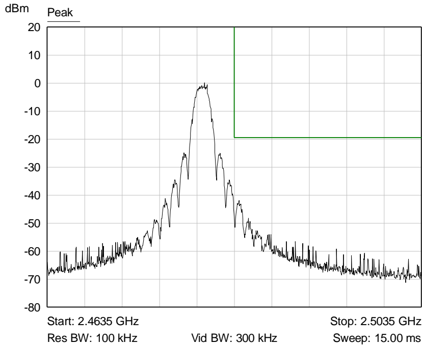
Graph 34: Upper Band Edge Plot
