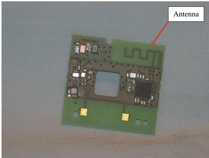
Photograph 18: View of the Back Side of the PCB
