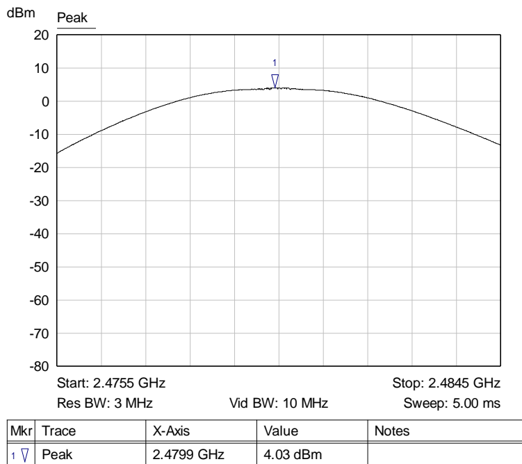
Graph 19: Highest Channel Output Power Plot
