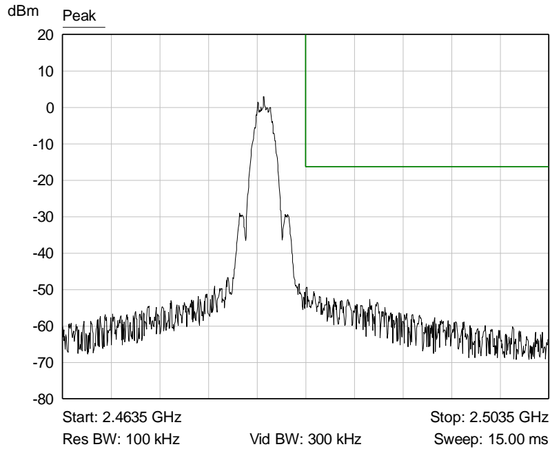
Graph 21: Upper Band Edge Plot
