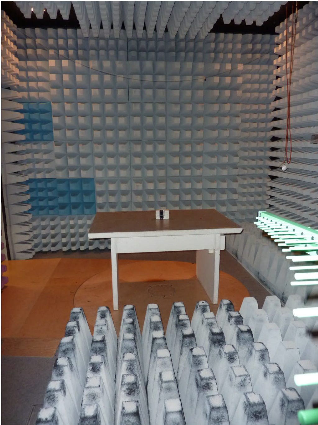
112808_a.JPG: PTM210 C, test setup fully anechoic chamber
