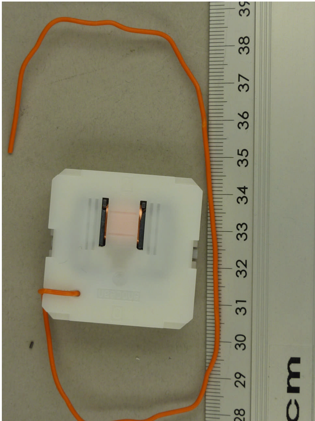
112808_4.JPG: PTM210 C, internal (bottom) view, unmodified sample
