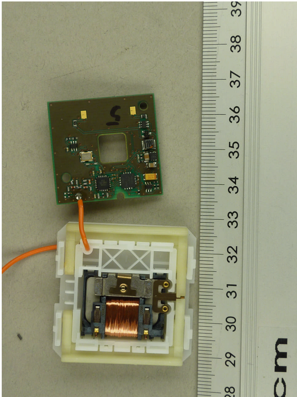
112808_5.JPG: PTM210 C, internal view
