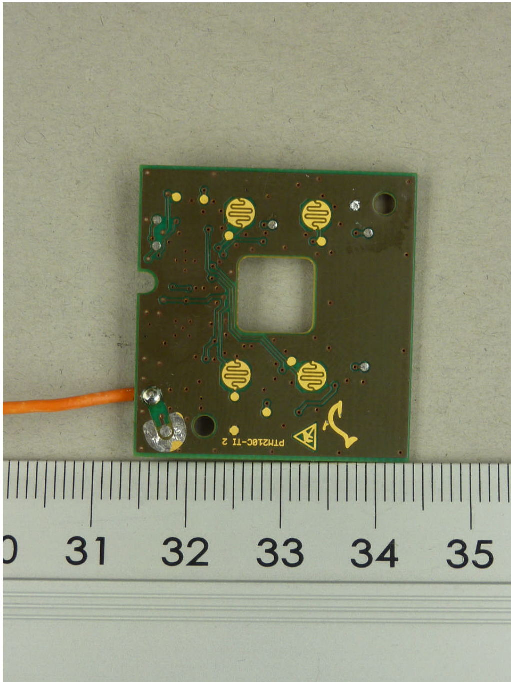
112808_6.JPG: PTM210 C, PCB, top view
