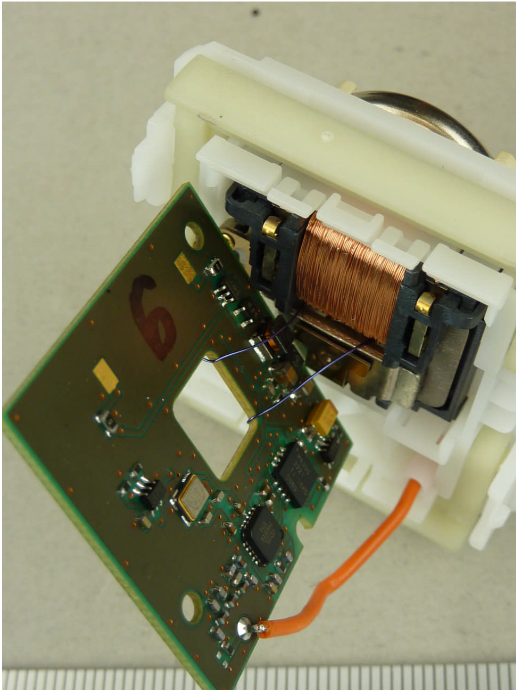
112808_12.JPG: PTM210 C, internal view, modified sample
