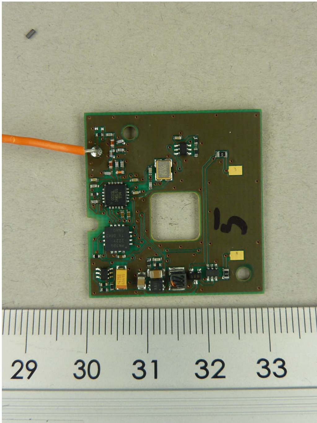
112808_10.JPG: PTM210 C, PCB, bottom view
