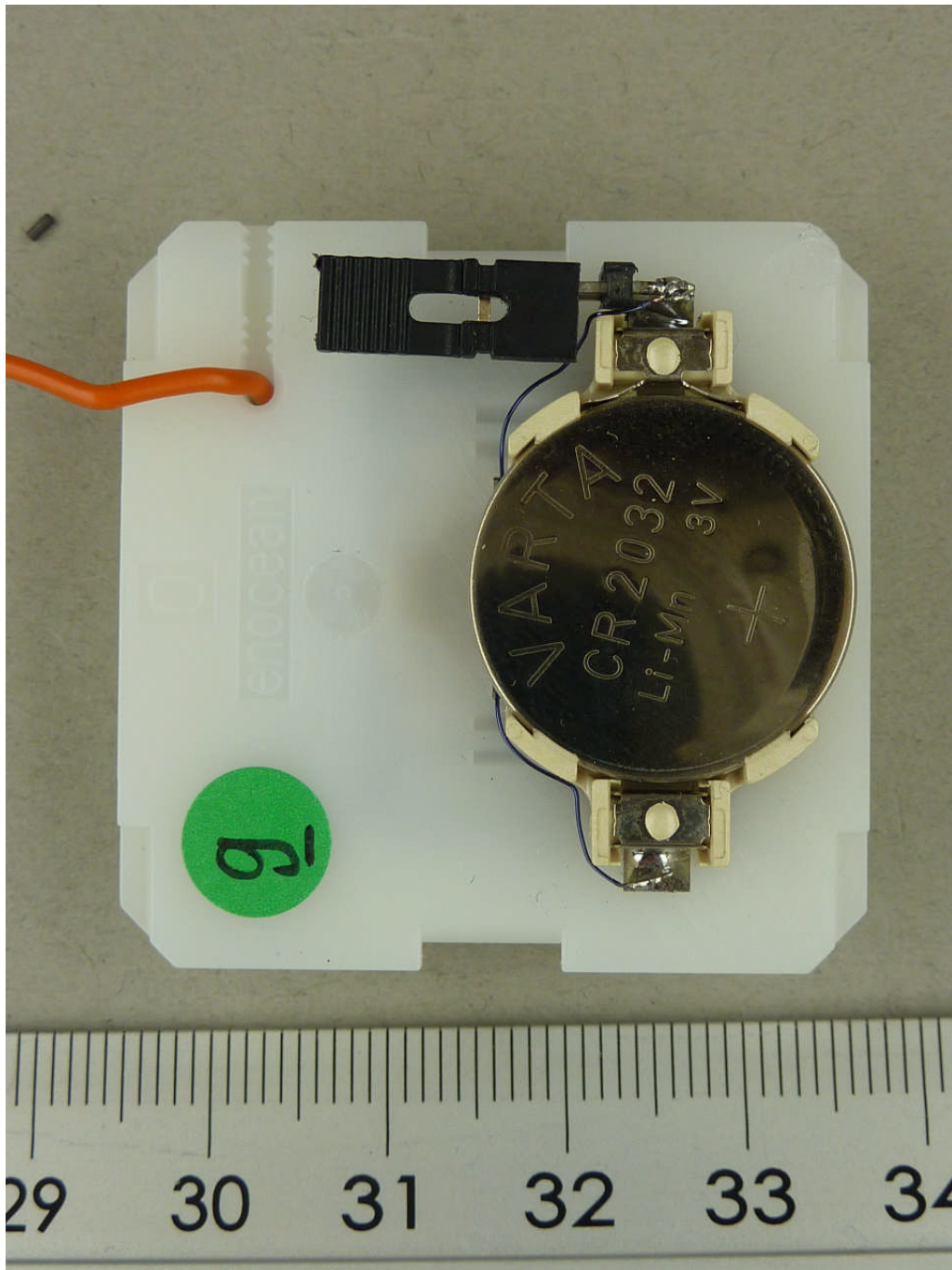
112808_11.JPG: PTM210 C, internal (bottom) view, modified sample
