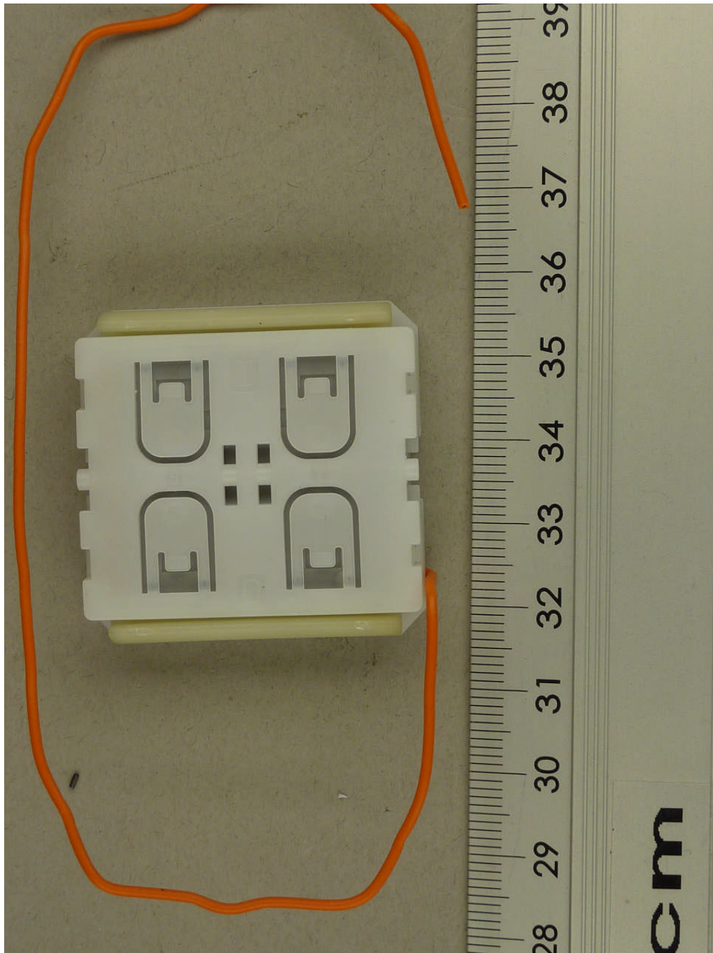
112808_3.JPG: PTM210 C, internal (top) view
