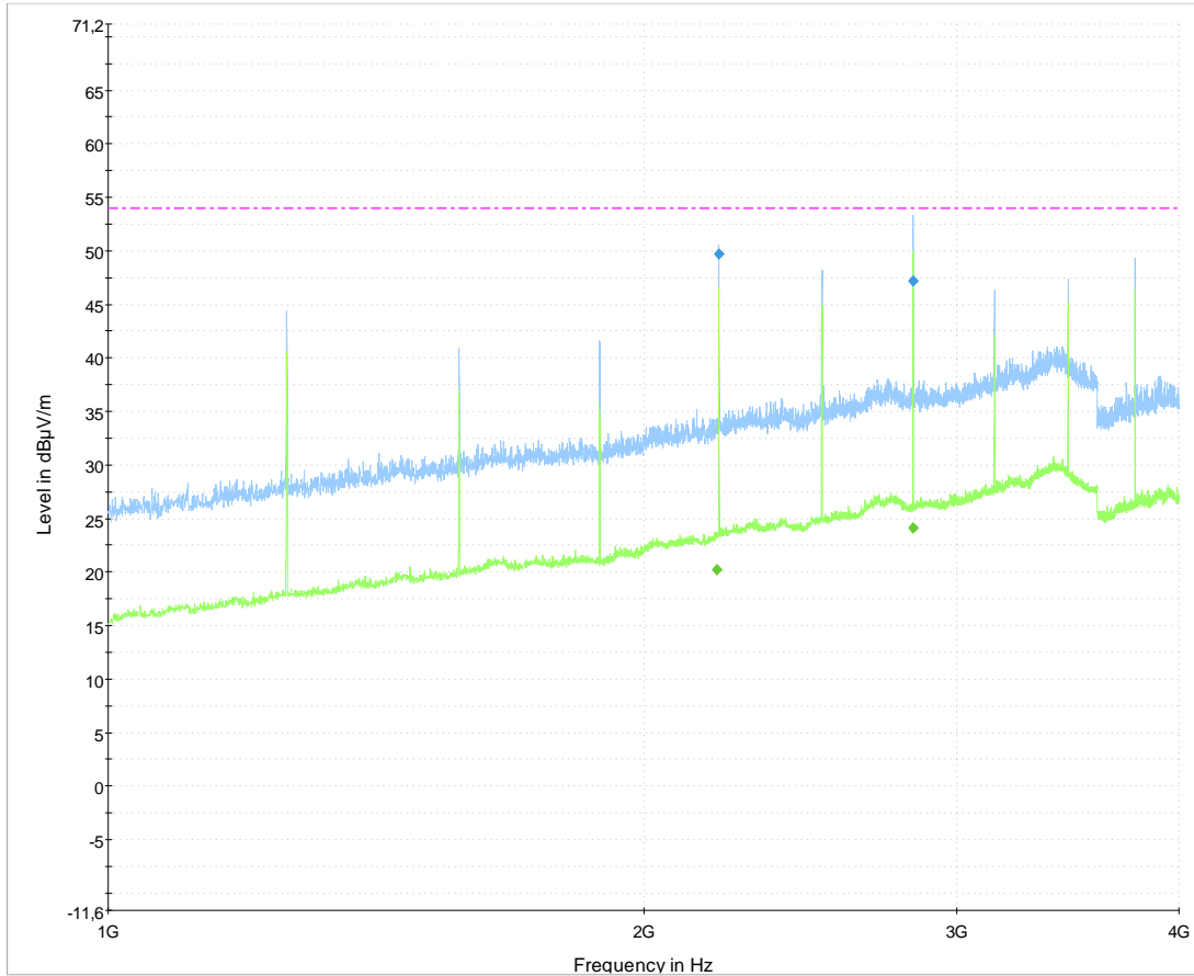
Figure 6-10: Radiated Emissions (1GHz – 4GHz)
