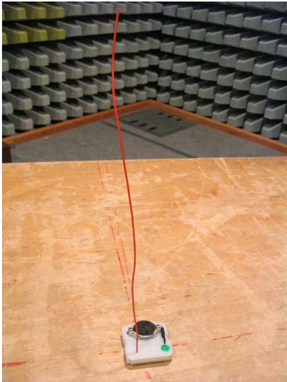
Figure 4-1: Photos of EUT
