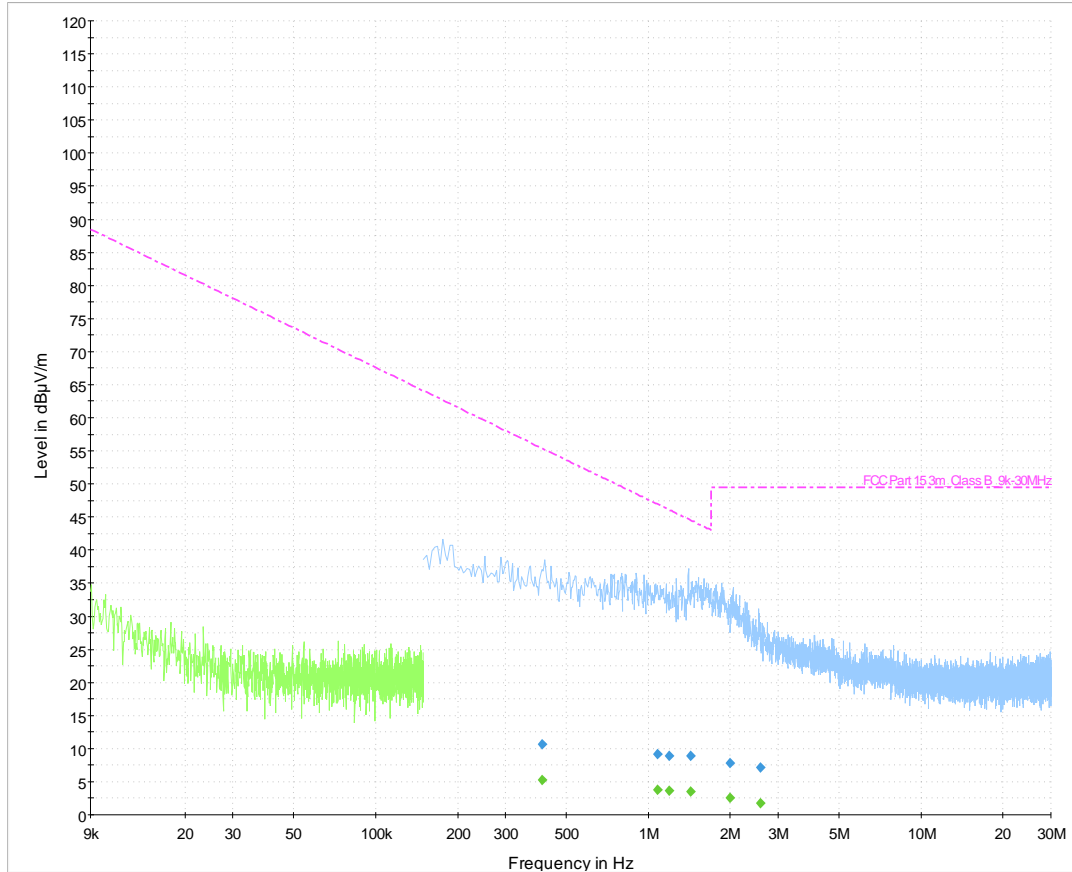
Figure 6-6: Radiated Emissions (9kHz – 30MHz)
