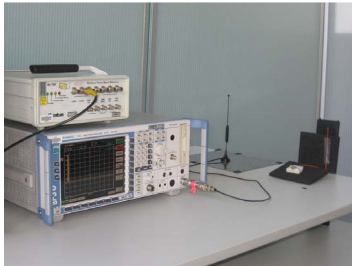
Figure 6-11: Test Configuration – Emission Bandwidth
