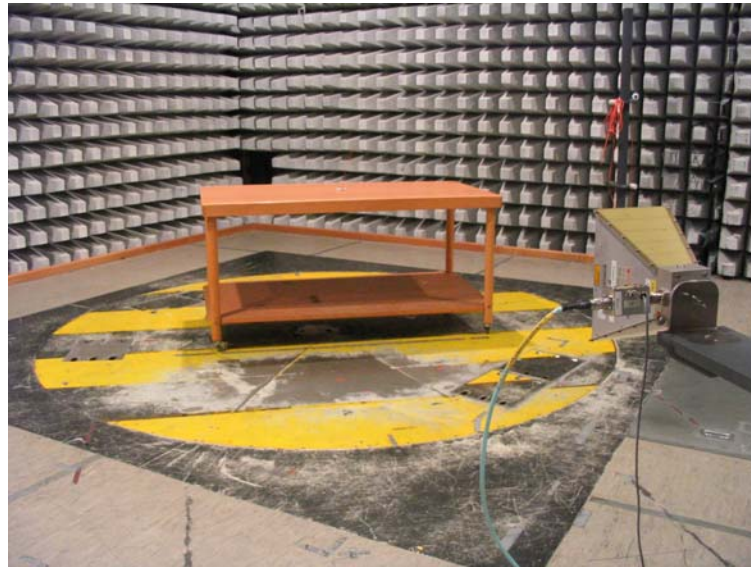
Figure 6-9: Test Configuration – Radiated Emissions (1GHz – 4GHz)
