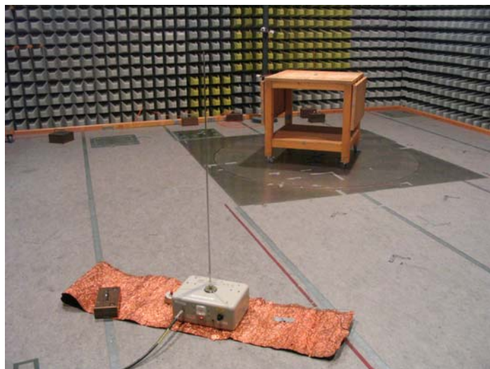
Figure 6-5: Test Configuration – Radiated Emissions (9kHz – 30MHz)
