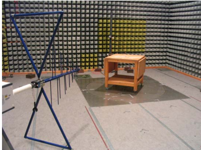
Figure 6-4: Test Configuration – Field Strength of Fundamental Wave
