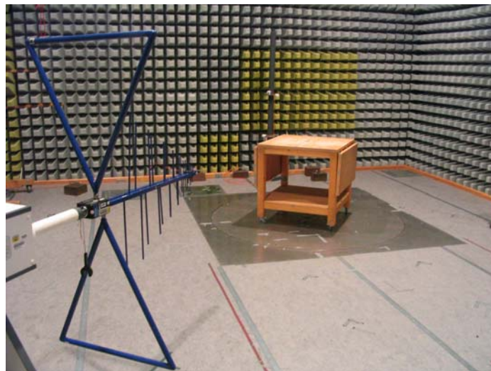
Figure 6-7: Test Configuration – Radiated Emissions (30MHz – 1GHz)
