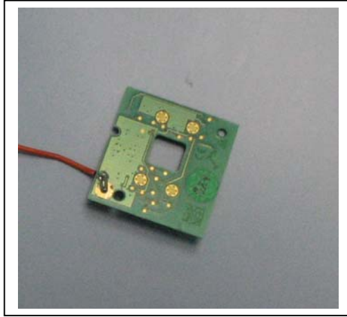
Fig. 4: PCB bottom view
