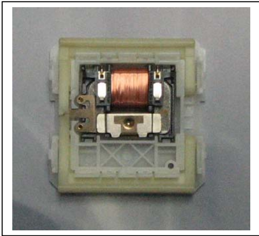
Fig. 1: Bottom Case including ECO200 and Energy Bows
