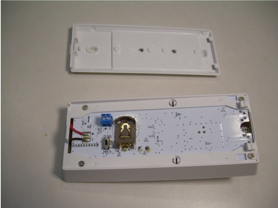
Photograph 5 – View of the EUT with Back Cover Removed
