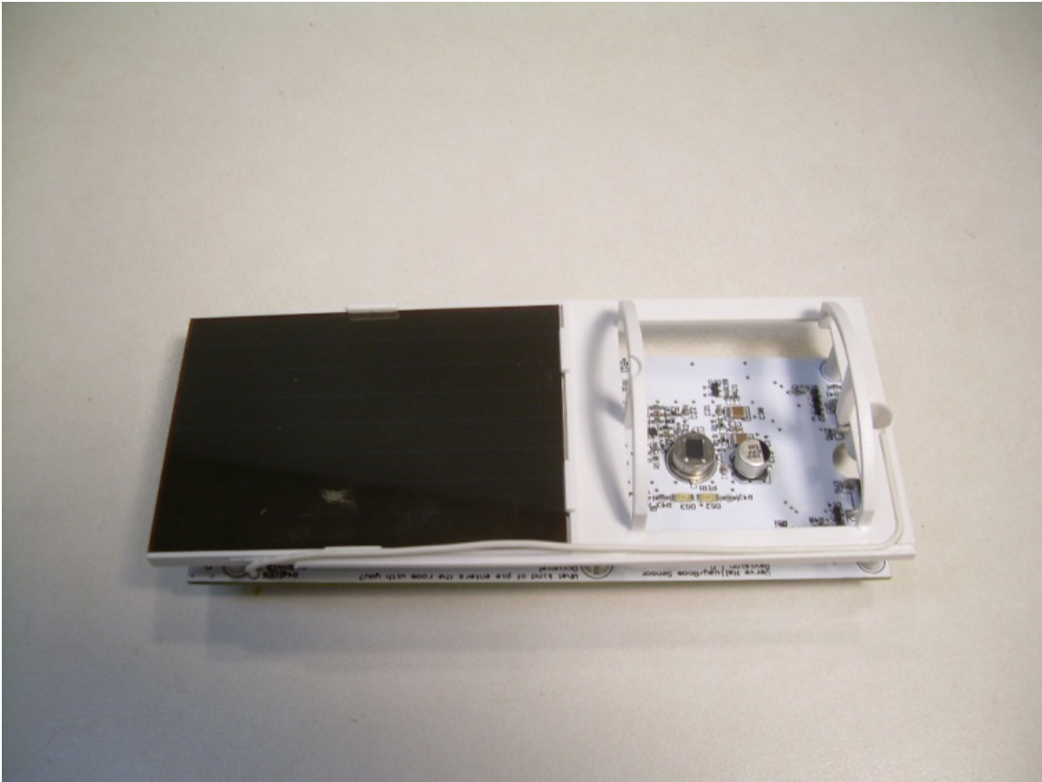
View of the EUT with Front Cover Removed
