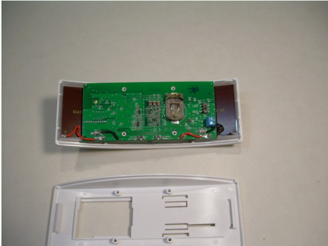
View of the EUT and back of PCB with Back Cover Removed
