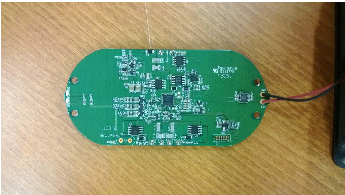
Photograph 4: WLS1_PCB top
