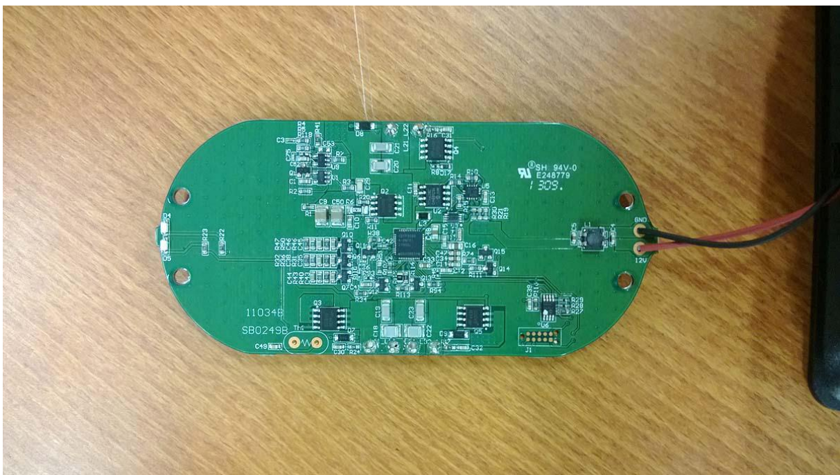
Photograph 4: WLS1_PCB top
