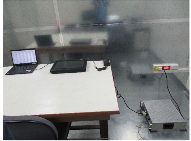
Part_15.247_LE_Conduction_Setup
