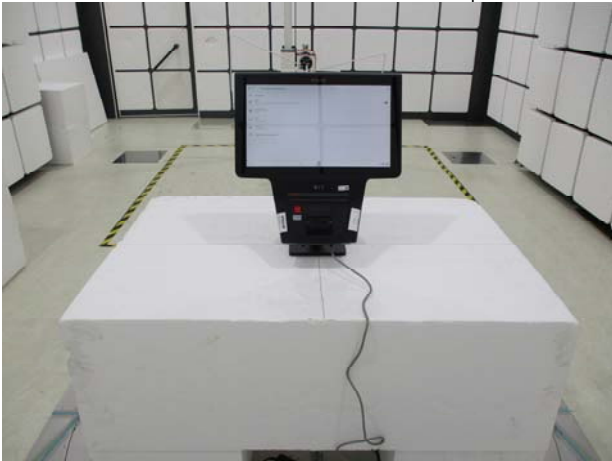
P15.225_NFC_Radiated_variant_Setup
