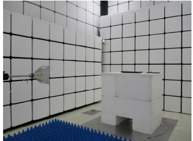
Part_15.247_BT_Radiated_variant_Setup
