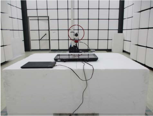
Part_15.247_LE_Radiated_Setup
