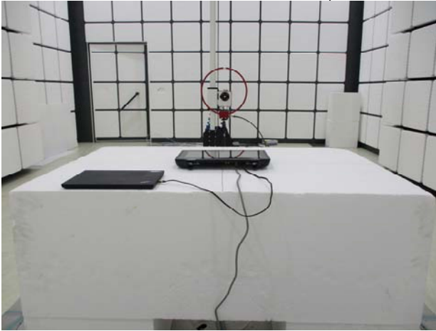
Part_15.247_WLAN_Radiated_variant_Setup
