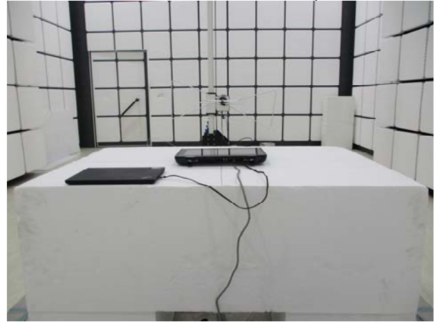
Part_15.247_LE_Radiated_variant_Setup
