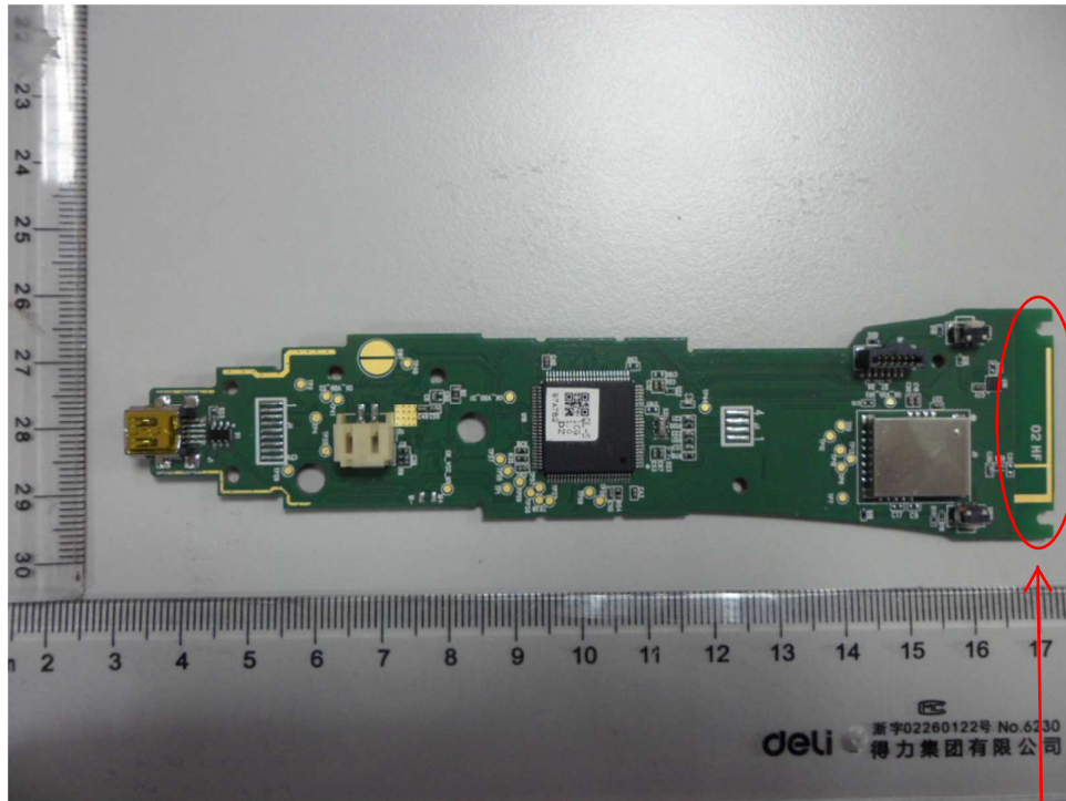
Main Board side A
