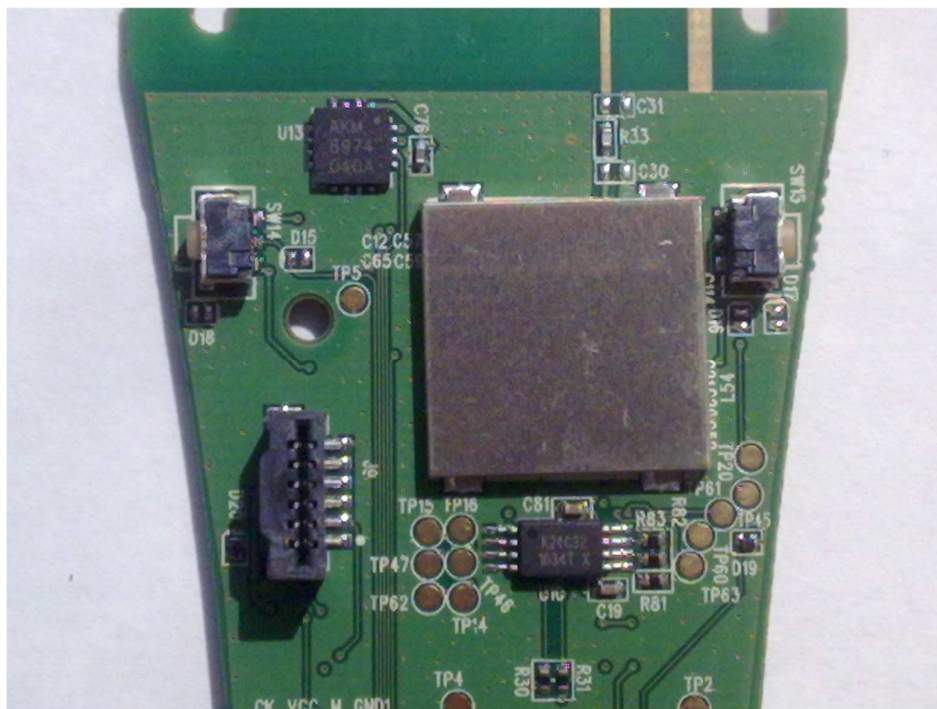
RF Board Side A with Shield
