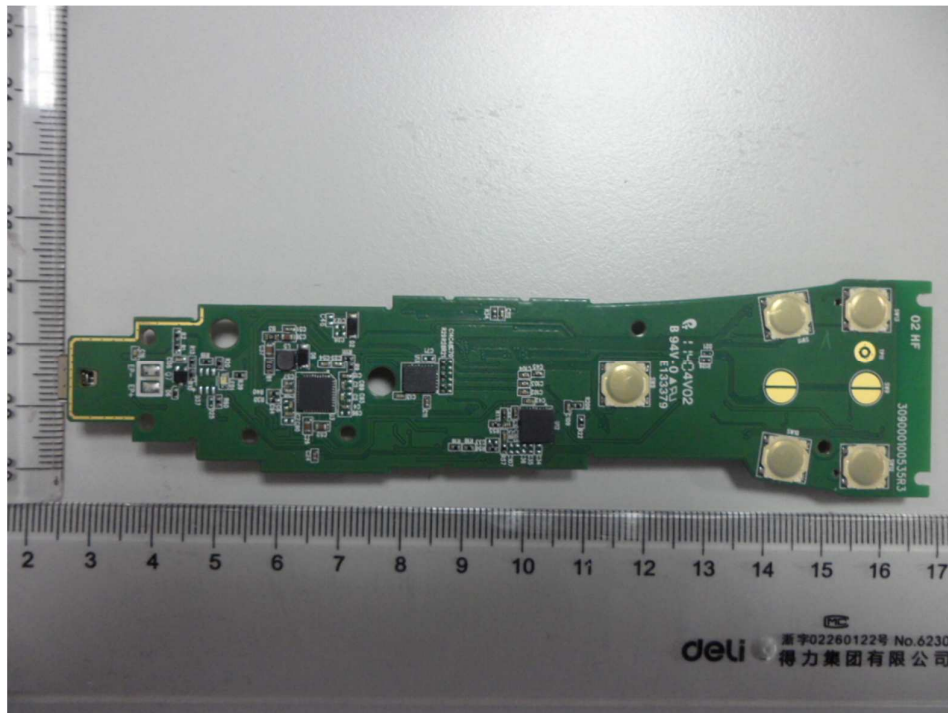
Main Board side B
