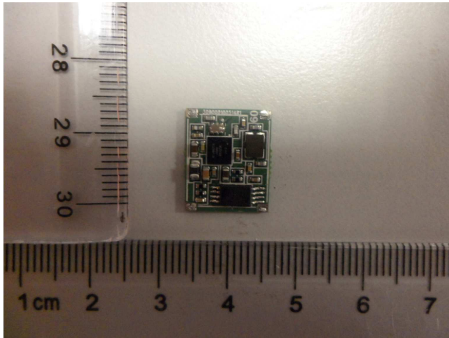
RF Board Side A without Shield
