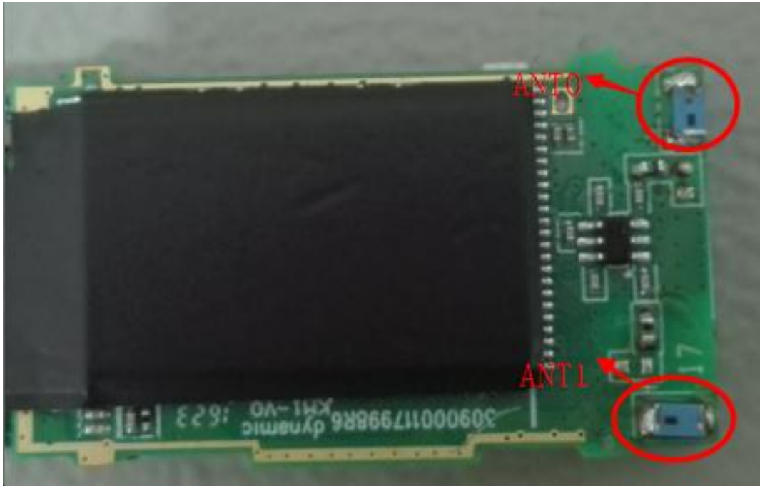
(7) EUT Photo
