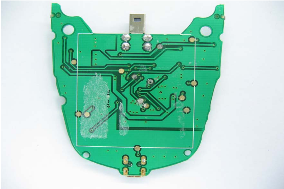
Internal View of EUT – 3 (Car Kit Base)
