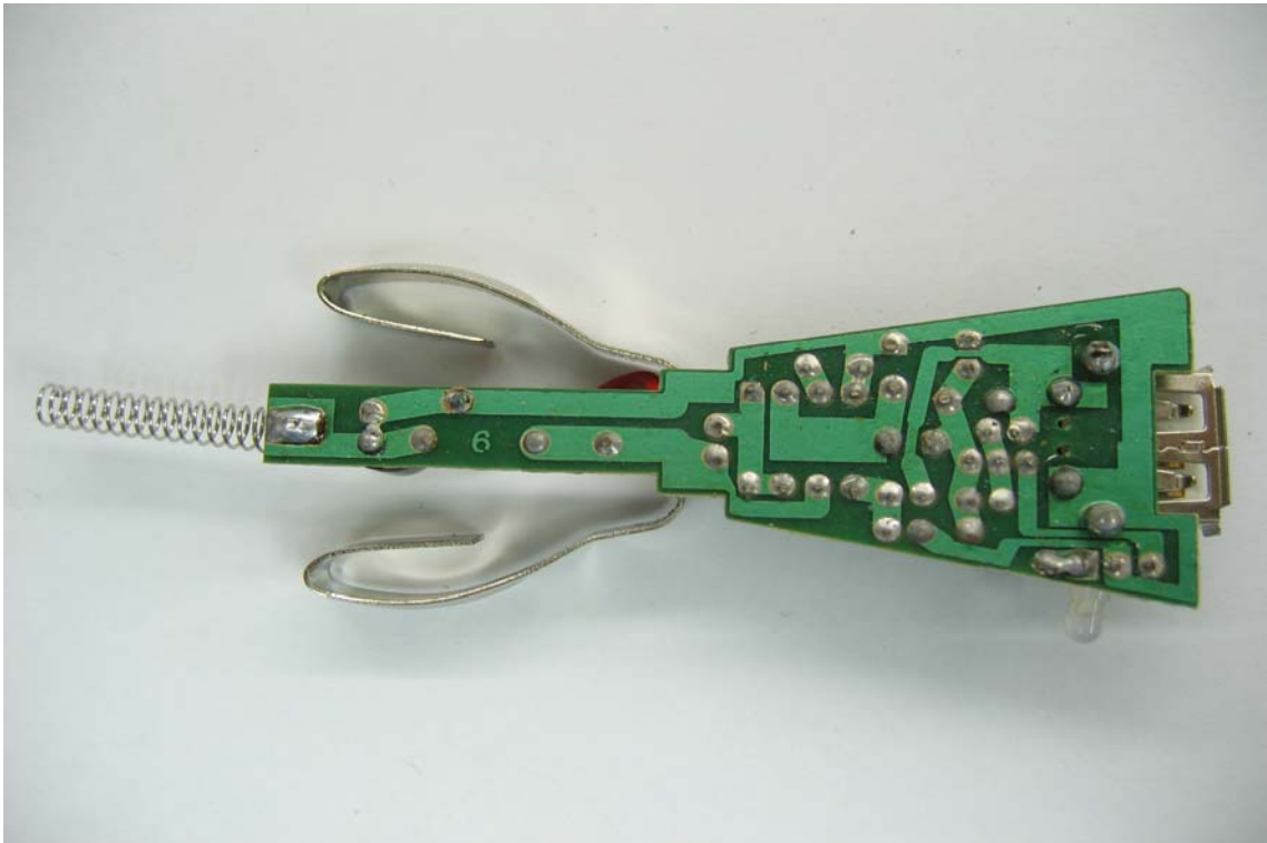
Internal View of EUT – 2 (Car Adaptor)
