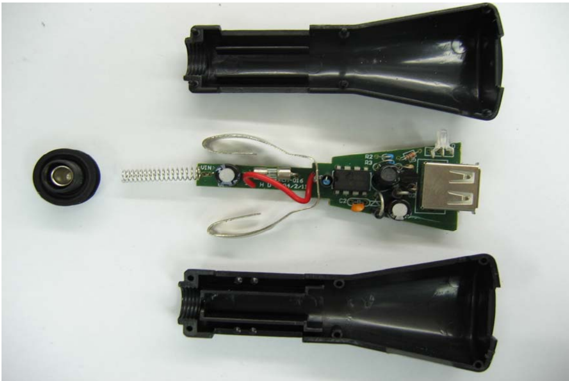
Open View of EUT (Car Adaptor)
