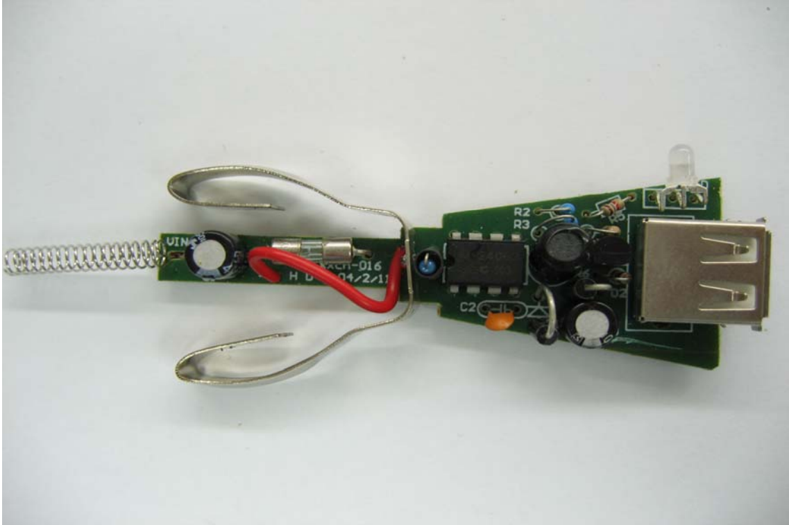
Internal View of EUT – 1 (Car Adaptor)
