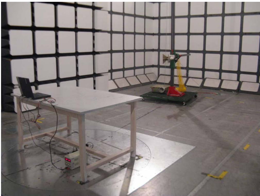
Transmitting Mode: Radiated Emissions - Rear View (Above 1GHz)
