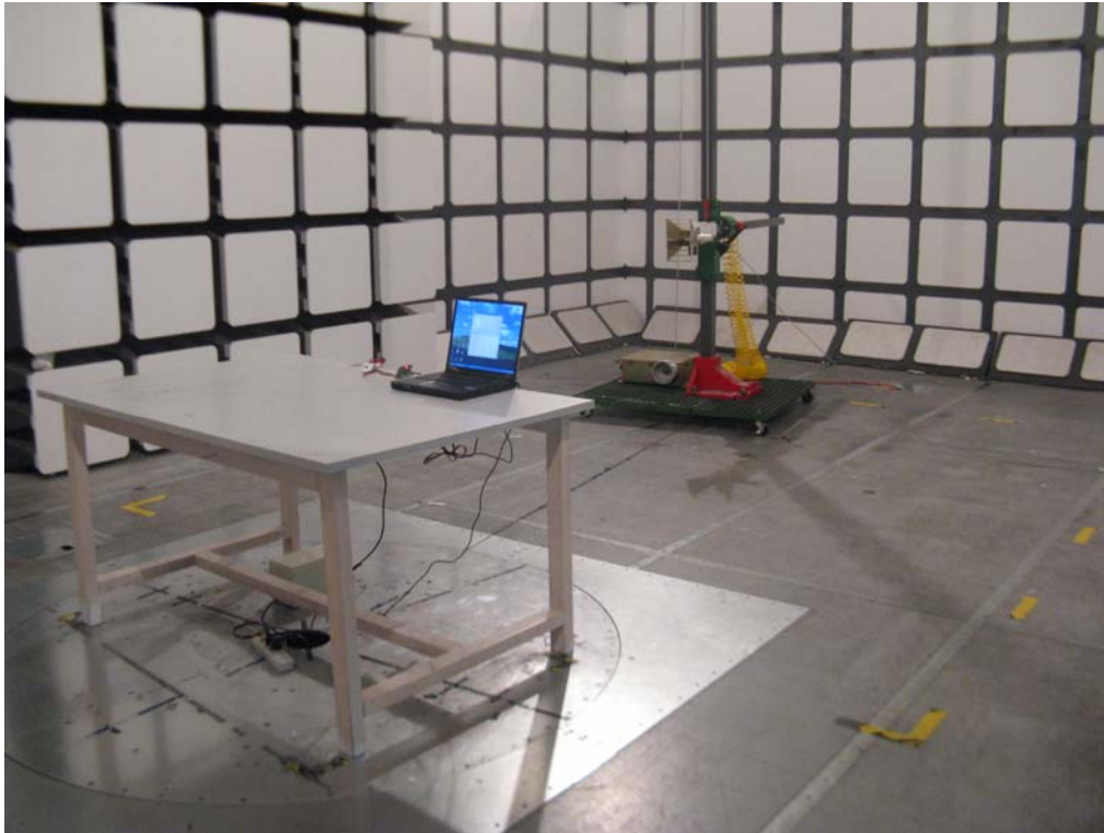
Transmitting Mode: Radiated Emissions - Front View (Above 1GHz)
