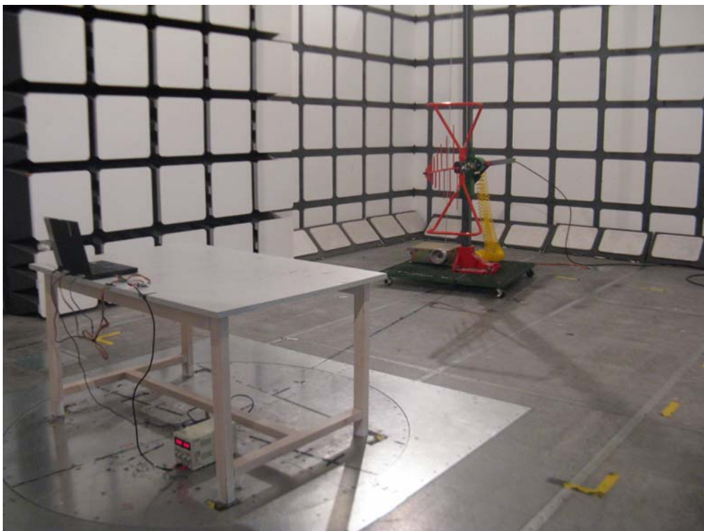
Transmitting Mode: Radiated Emissions - Rear View (30-1000 MHz)
