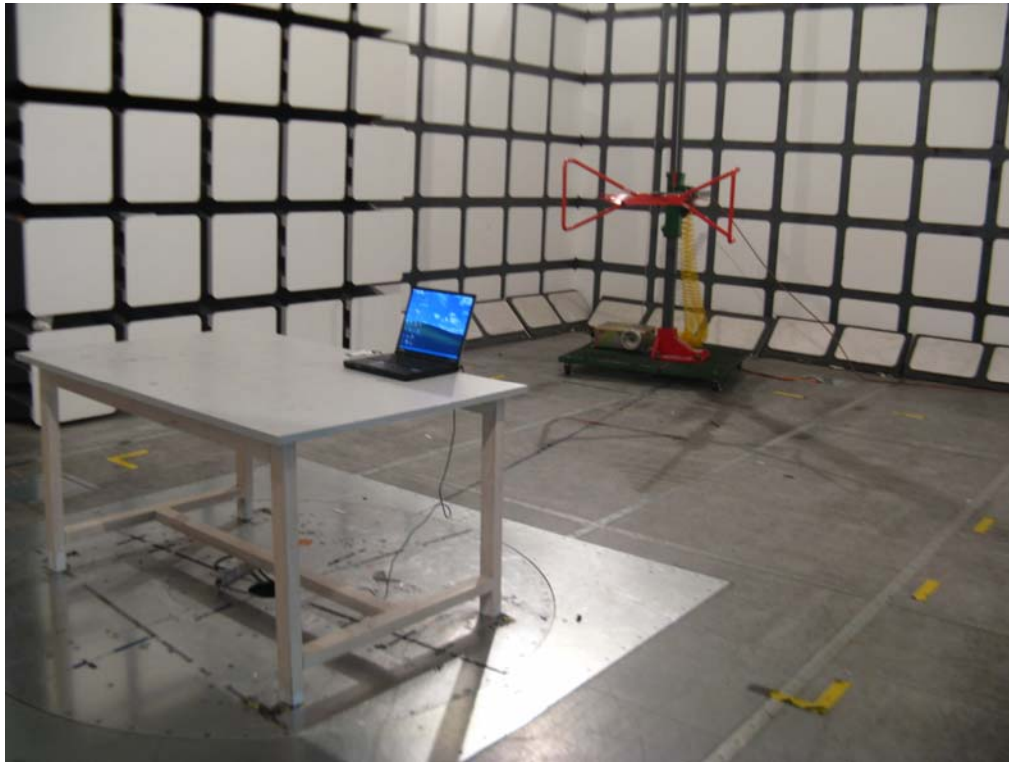
Charging Mode: Radiated Emissions - Front View (30-1000MHz)
