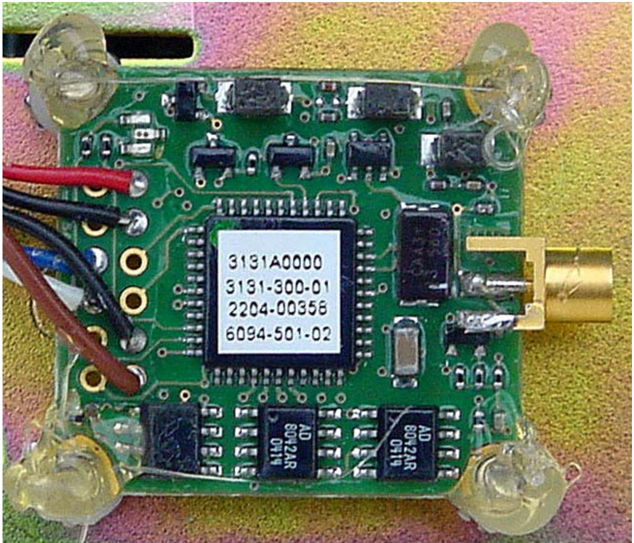
Antenna Driver Board – Front
