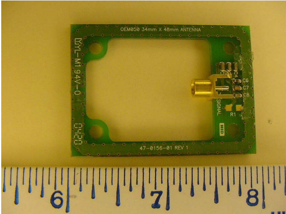
Antenna Top
