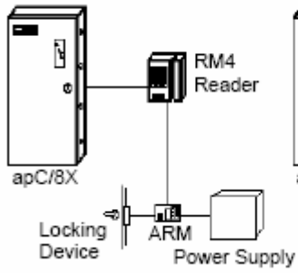
apC/8X to Magnetic Reader
