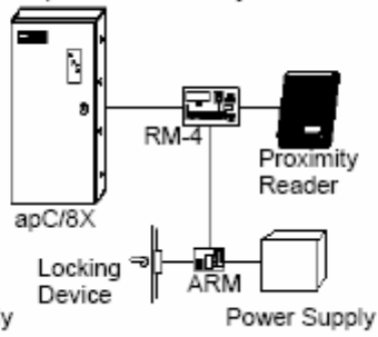
apC/8X to Proximity Reader
