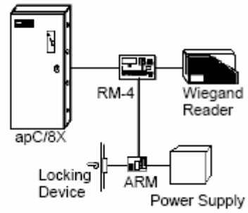
apC/8X to Wiegand Reader
